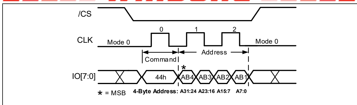
Figure 15-2b. Erase Security Registers Command (ODDR Mode) A 32-Bit Address is required when the device is operating in ODDR mode
