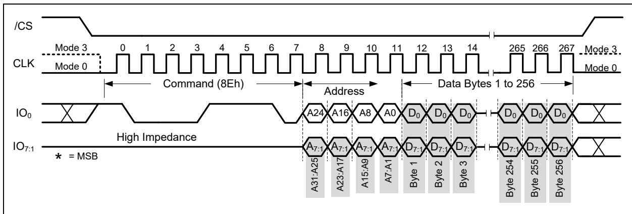
Figure 11-6. Page Program Octal Address/Data with 4-Byte Addr. (SDR Mode)
