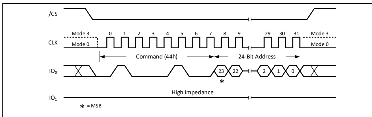
Figure 15-2a. Erase Security Registers Command (SDR Mode) A 32-Bit Address is required when the device is operating in 4-Byte Address Mode
