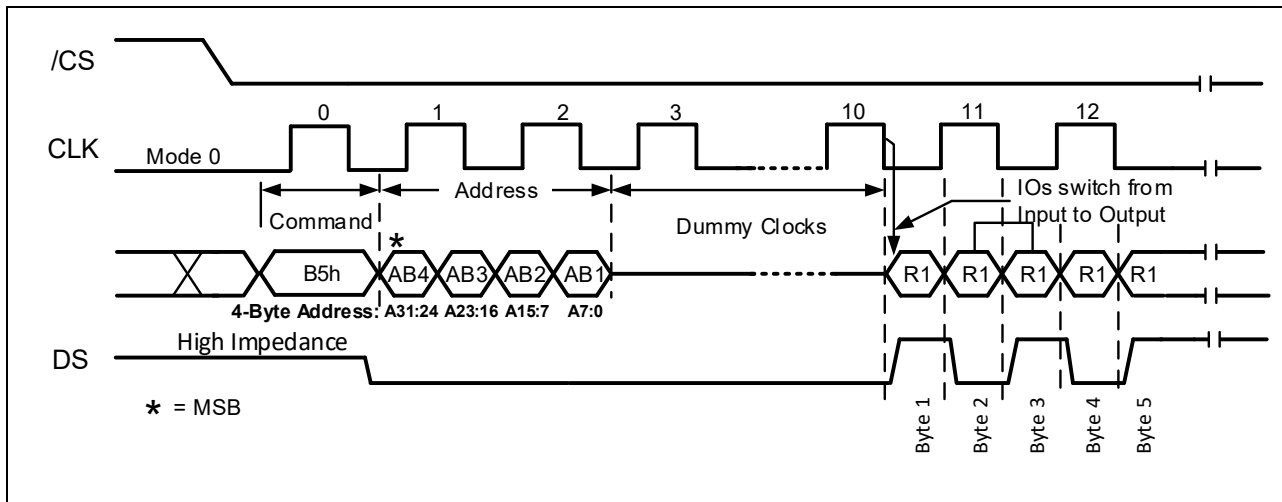
Figure 8-5b. Read Non-Volatile Configuration Register Command (ODDR Mode)
