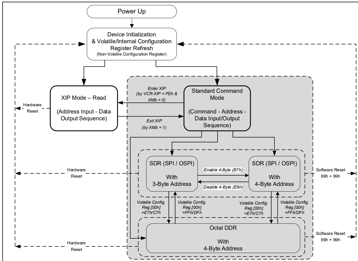
Figure 4-1. W35T64NW Serial Flash Memory Operation Diagram
