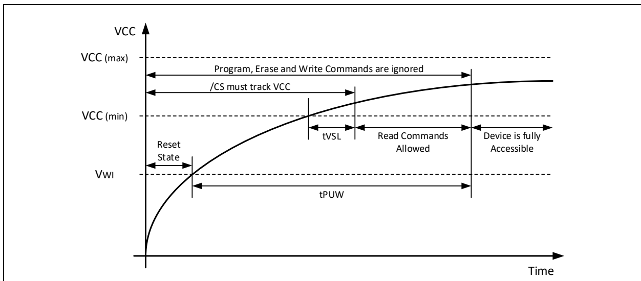
Figure 20-1. Power-up Timing and Voltage Levels
