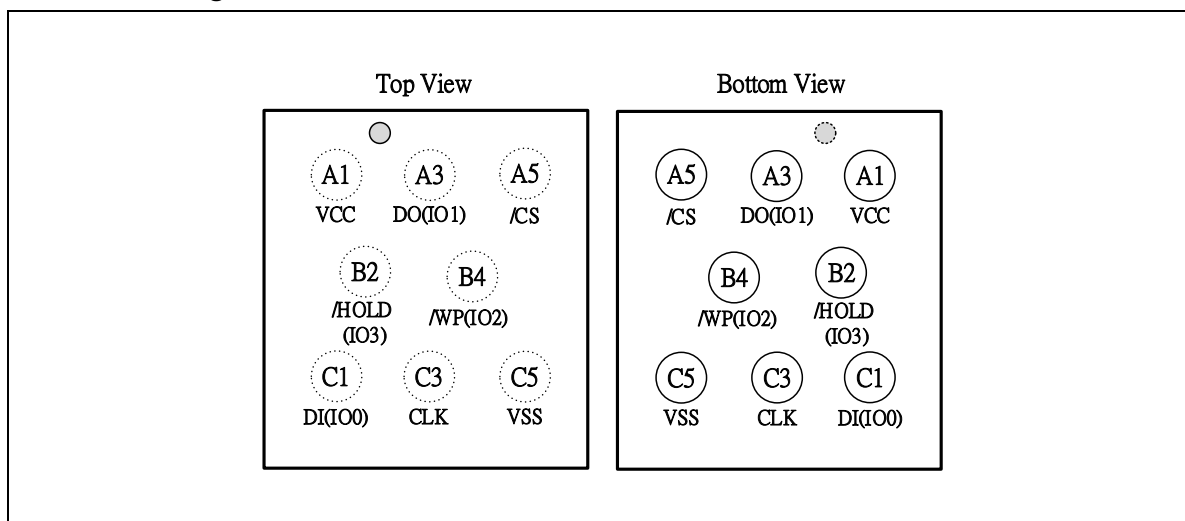
Figure 1d. W25Q80PW Ball Assignments, 8-ball WLCSP (Package Code BY)
