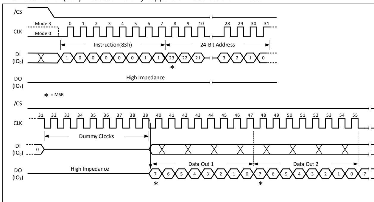
Figure 54c. Read Buffer
