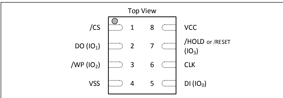
Figure 1b. W25Q80PW Pad Assignments, 8-pad WSON 6x5-mm (Package Code XH/ZT/UU)
