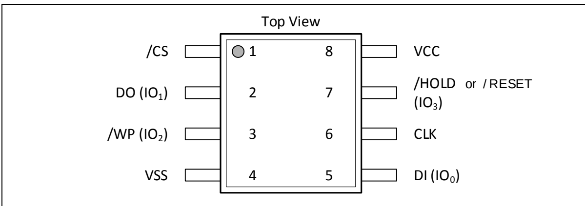
Figure 1a. W25Q80PW Pin Assignments, 8-pin SOP (Package Code SN/SS)
