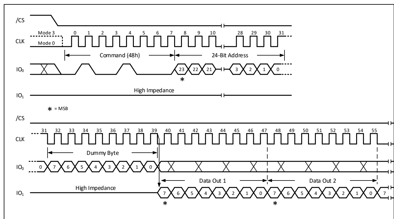
Figure 14-4a. Read Security Registers Command (SDR Mode)
