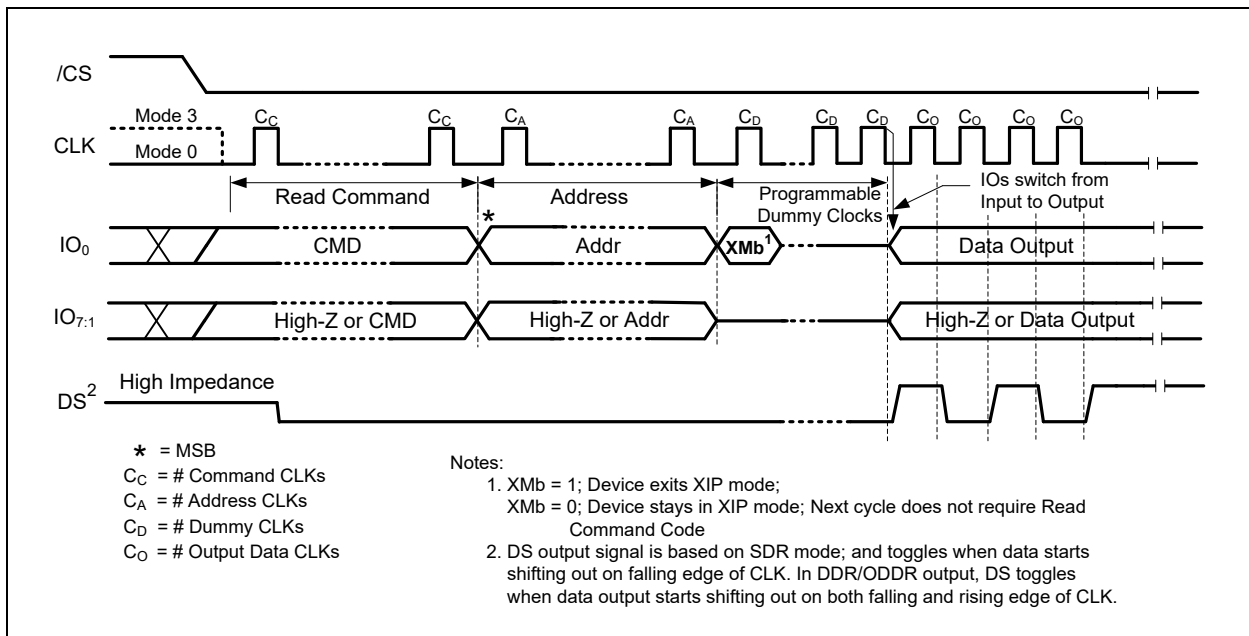
Figure 4-3. XIP Mode Entry From Volatile Configuration Register Address 06h (VCR-XIP)
