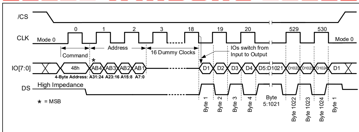
Figure 14-4b. Read Security Registers Command (ODDR Mode) A 32-Bit Address is required when the device is operating in ODDR Mode
