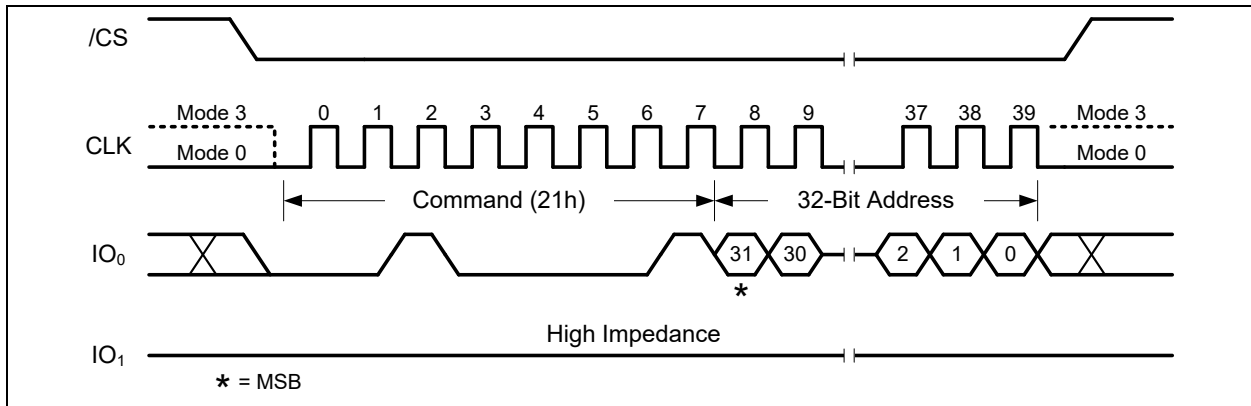
Figure 12-2. Sector Erase with 4-Byte Address Command (SDR Mode)
