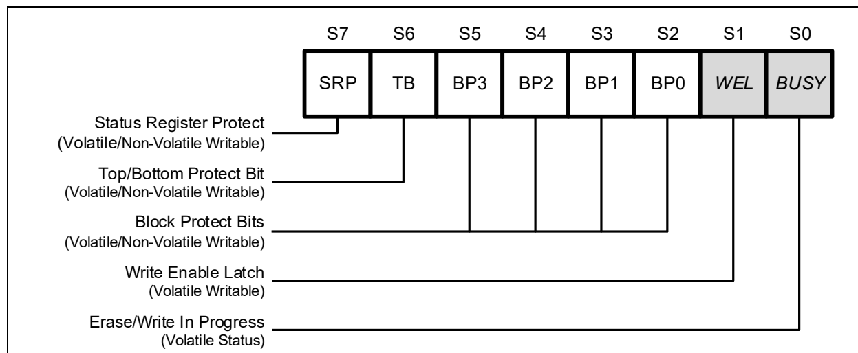
Figure 5-1. Status Register
