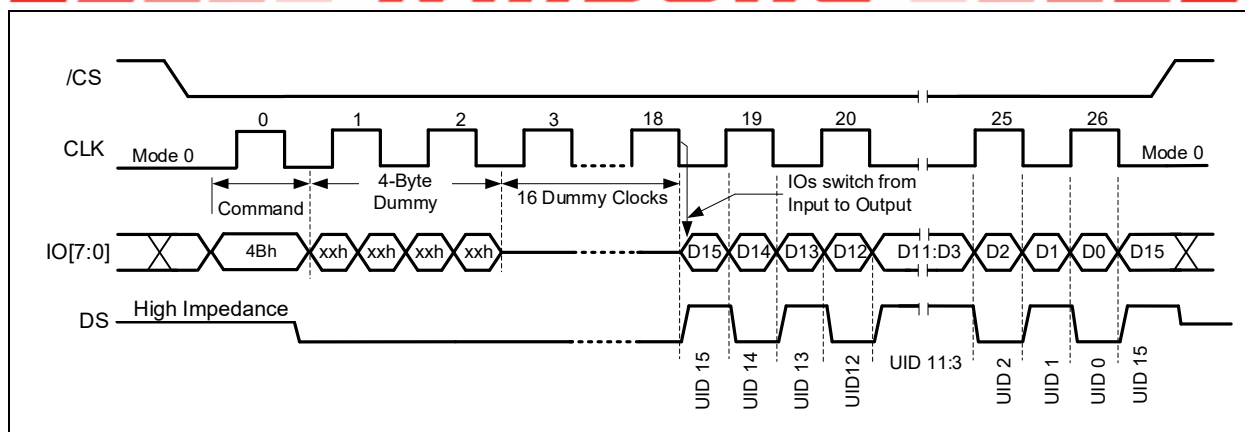
Figure 14-1b. Read Unique ID Command (ODDR Mode)
