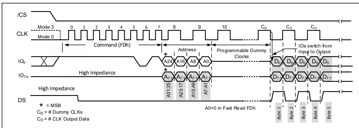
Figure 10-10. Fast Read DDR Octal I/O with 4-Byte Address (1-8d-8d SDR Mode)
