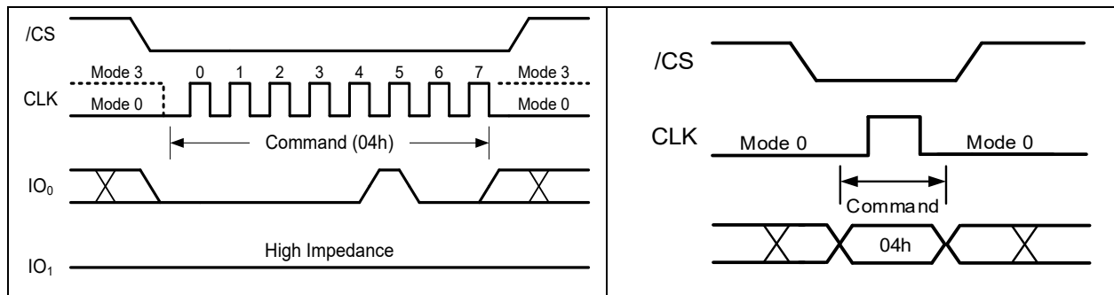
Figure 8-10. Write Disable Command for SDR Mode (left) or ODDR Mode (right)
