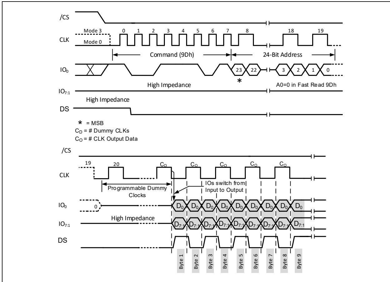
Figure 10-9. Fast Read DDR Single-Address-Input and Octal-Output (1-1d-8d SDR Mode)
