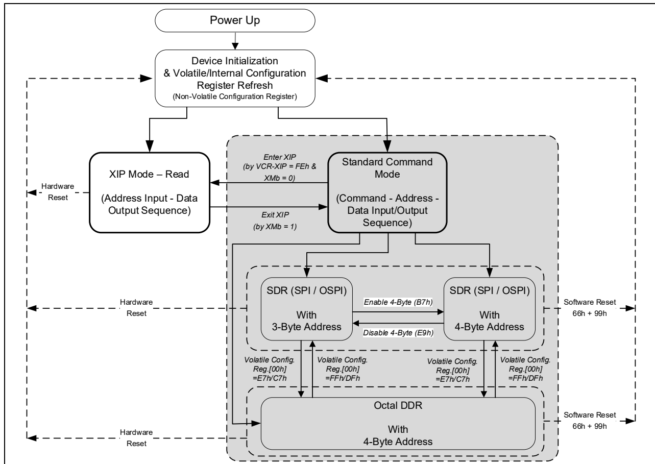
Figure 4-1. W35T02NW Serial Flash Memory Operation Diagram
