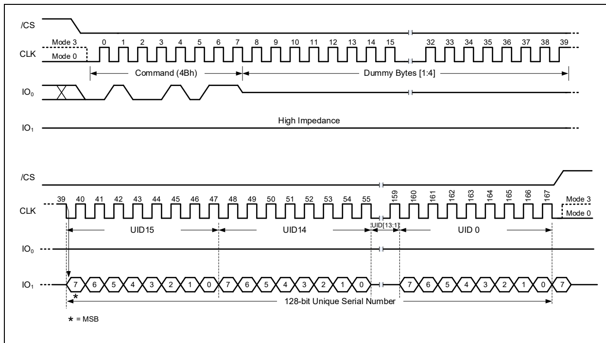
Figure 14-1a. Read Unique Command (SDR Mode)
