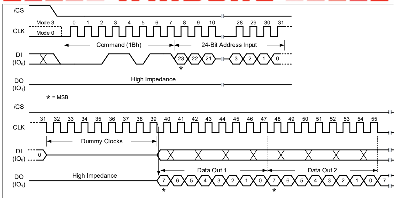
Figure 18-3a. Read 8-Byte CRC Code Command Sequence (1-1-1 SDR Mode) A 32-Bit Address is required when the device is operating in 4-Byte Address Mode
