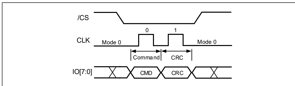
Figure 18-4a. 8d-0-0 CRC-In-Transit Command Protocol (ODOR Mode)
