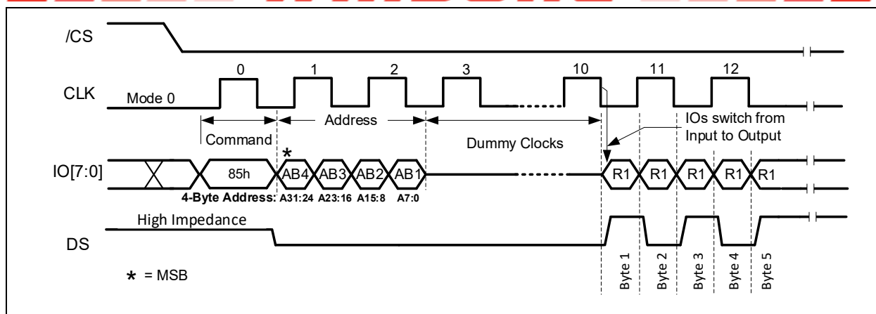
Figure 8-7b. Read Volatile Configuration Register Command (ODDR Mode)
