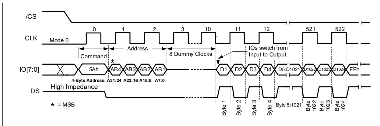
Figure 7-2b. Read SFDP Register Command Sequence (ODDR Mode) A 32-Bit Address is required when the device is operating in Odd Mode
