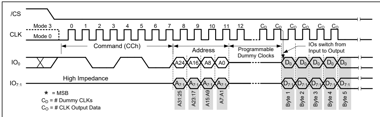
Figure 10-8. Fast Read Octal I/O Command using 4-Byte Address (1-8 SDR)
