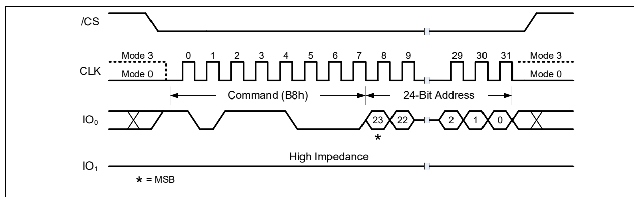
Figure 17-6a. (1-1-0) Erase DLP Register Command (1-1-0 SDR Mode) A 32-Bit Address is required when the device is operating in 4-Byte Address Mode
