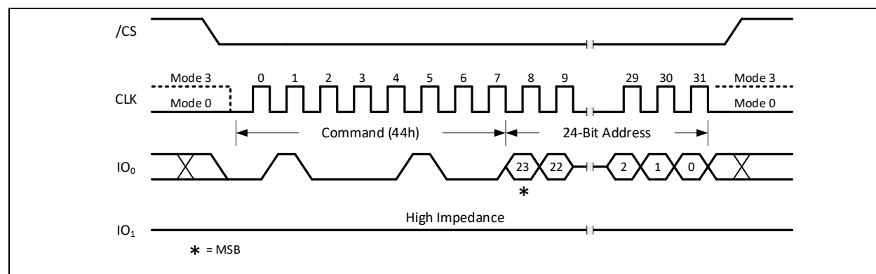
Figure 14-2a. Erase Security Registers Command (SDR Mode) A 32-Bit Address is required when the device is operating in 4-Byte Address Mode
