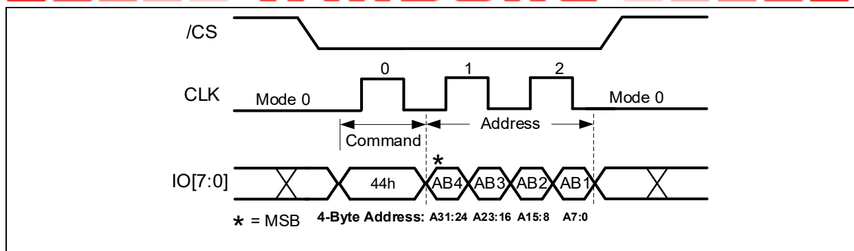
Figure 14-2b. Erase Security Registers Command (ODDR Mode)
