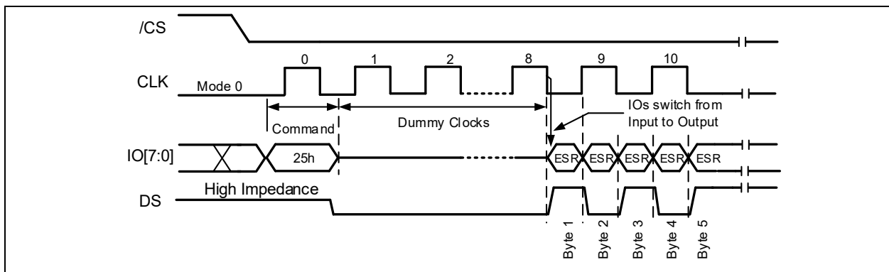
Figure 16-1b. Read ECC Status Register Command (ODDR Mode)
