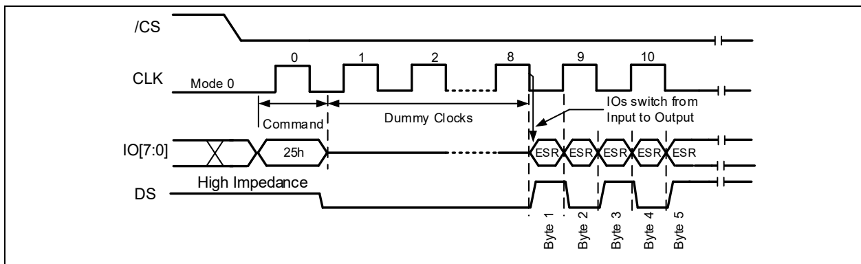
Figure 17-1b. Read ECC Status Register Command (ODDR Mode)
