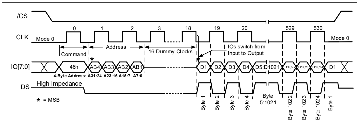
Figure 15-4b. Read Security Registers Command (ODDR Mode)
