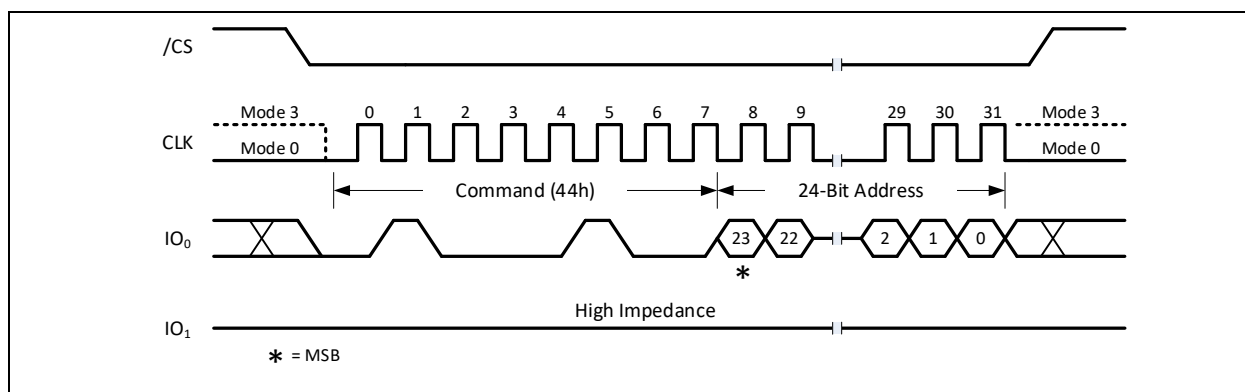
Figure 15-2a. Erase Security Registers Command (SDR Mode)
