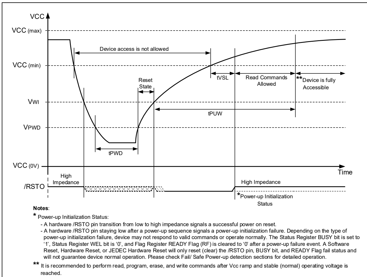
Figure 20-3. Power Cycle Requirement
