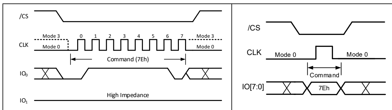
Figure 14-1. Global Block/Sector Lock Command for SDR Mode (left) or ODDR Mode (right)
