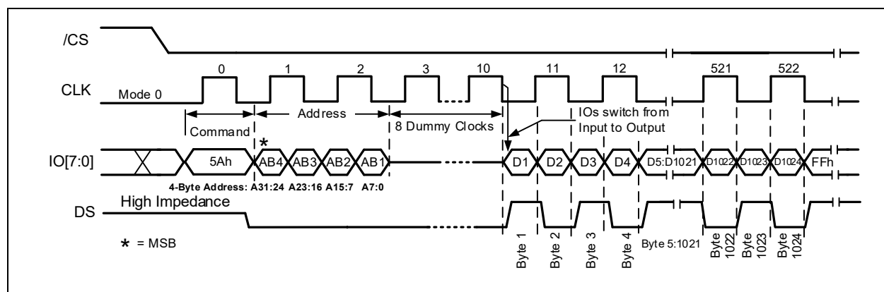
Figure 7-2b. Read SFD Register Command Sequence (ODDR Mode) A 32-Bit Address is required when the device is operating in ODDR Mode
