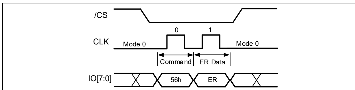
Figure 17-2b. Write ECC Status Register Command (ODDR Mode)
