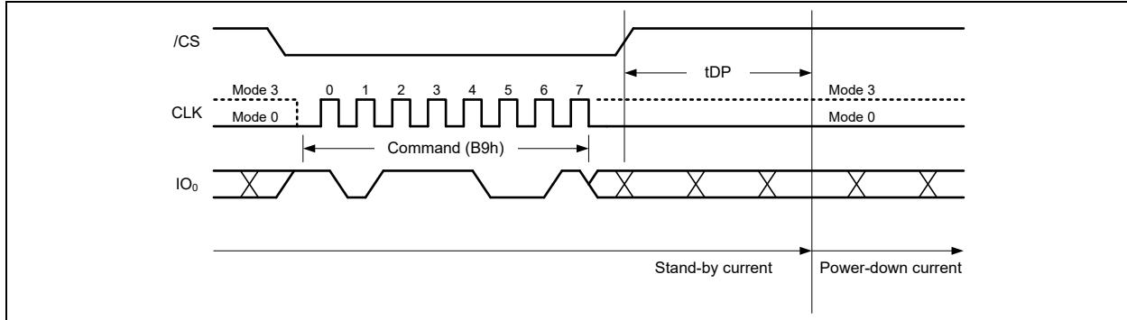
Figure 16-1a. Deep Power-down Command (SDR Mode)
