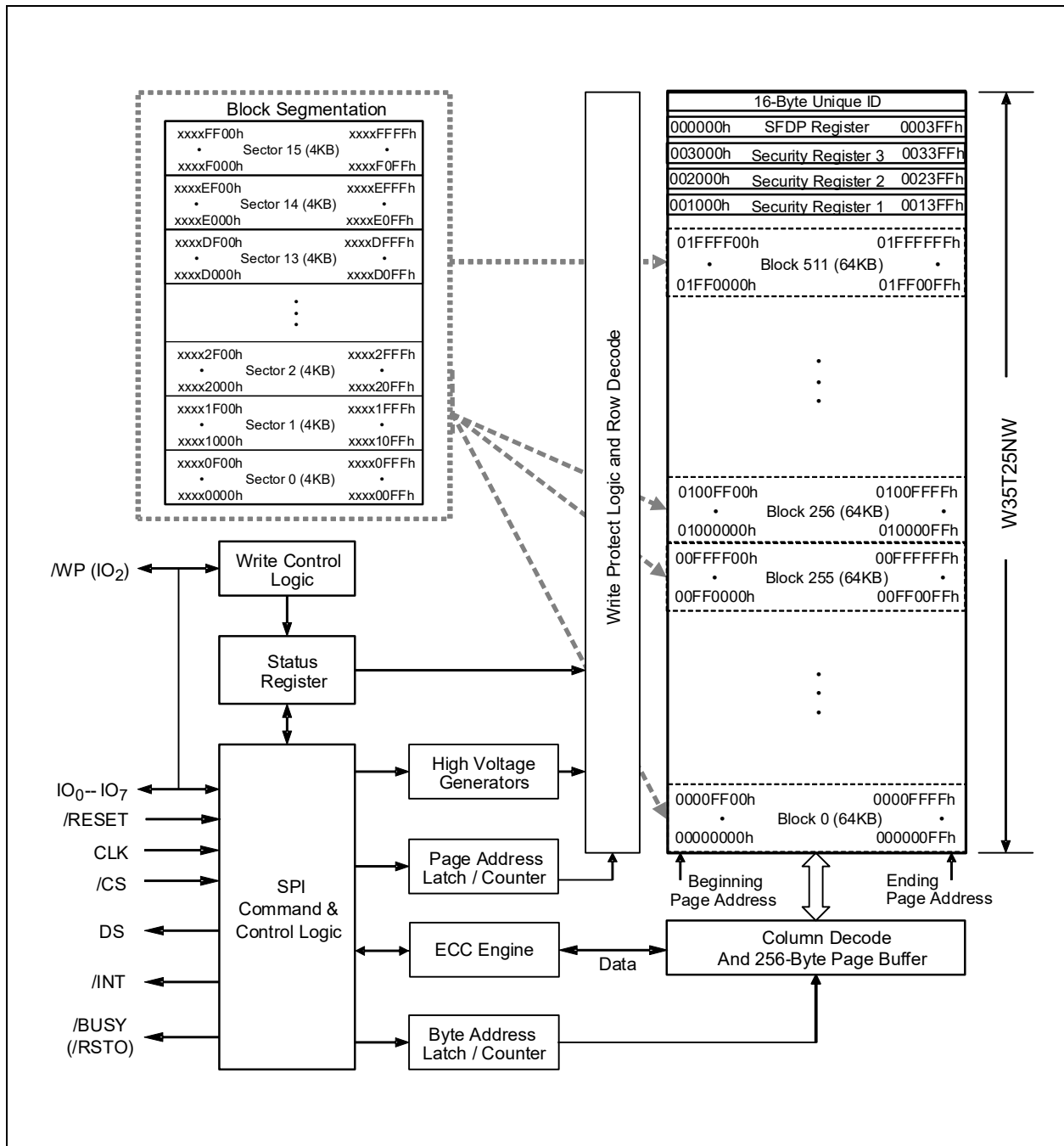
Figure 1. W35T25NW Serial Flash Memory Block Diagram
