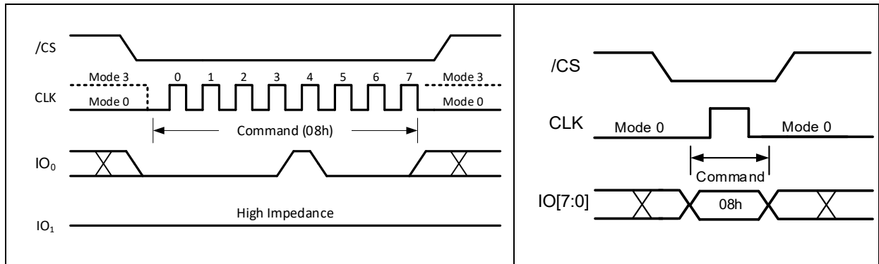
Figure 8-11. Write Enable for Volatile Status Register Command - SDR Mode (left) or ODDR Mode (right)
