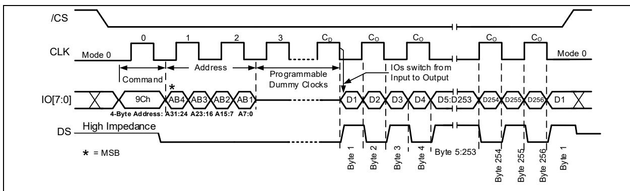
Figure 18-3b. (8d-8d-8d) Read DLP Command (ODDR Mode)
