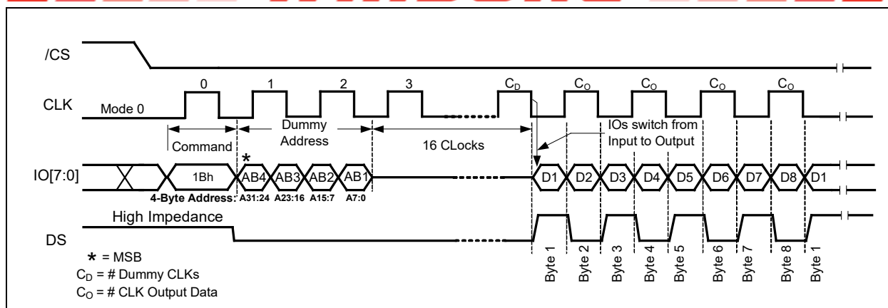
Figure 19-3b. ODDR Read 8-Byte CRC Code Command Sequence (ODDR Mode)
