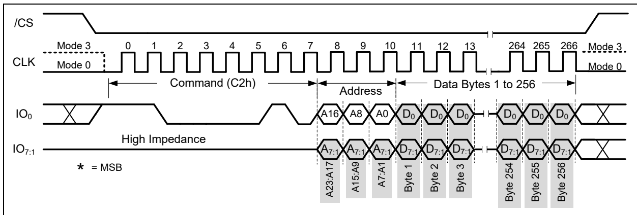
Figure 11-5. Page Program Octal Address/Data Command (SDR Mode) A 32-Bit Address is required when the device is operating in 4-Byte Address Mode
