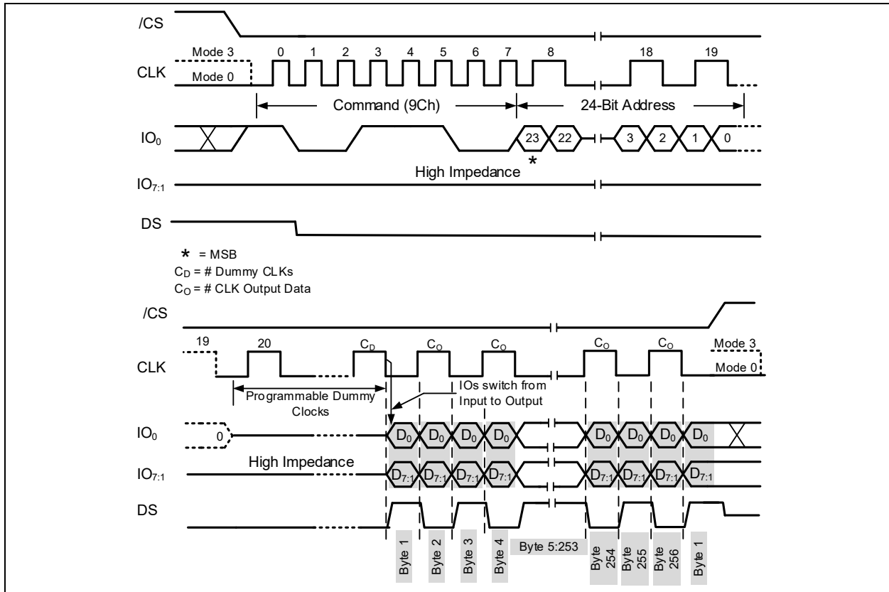
Figure 18-3a. (1-1d-8d) Read DLP Command (1-1d-8d SDR Mode) A 32-Bit Address is required when the device is operating in 4-Byte Address Mode
