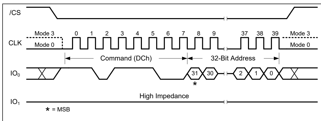
Figure 12-8. 64KB Block Erase with 4-Byte Address Command (SDR Mode)
