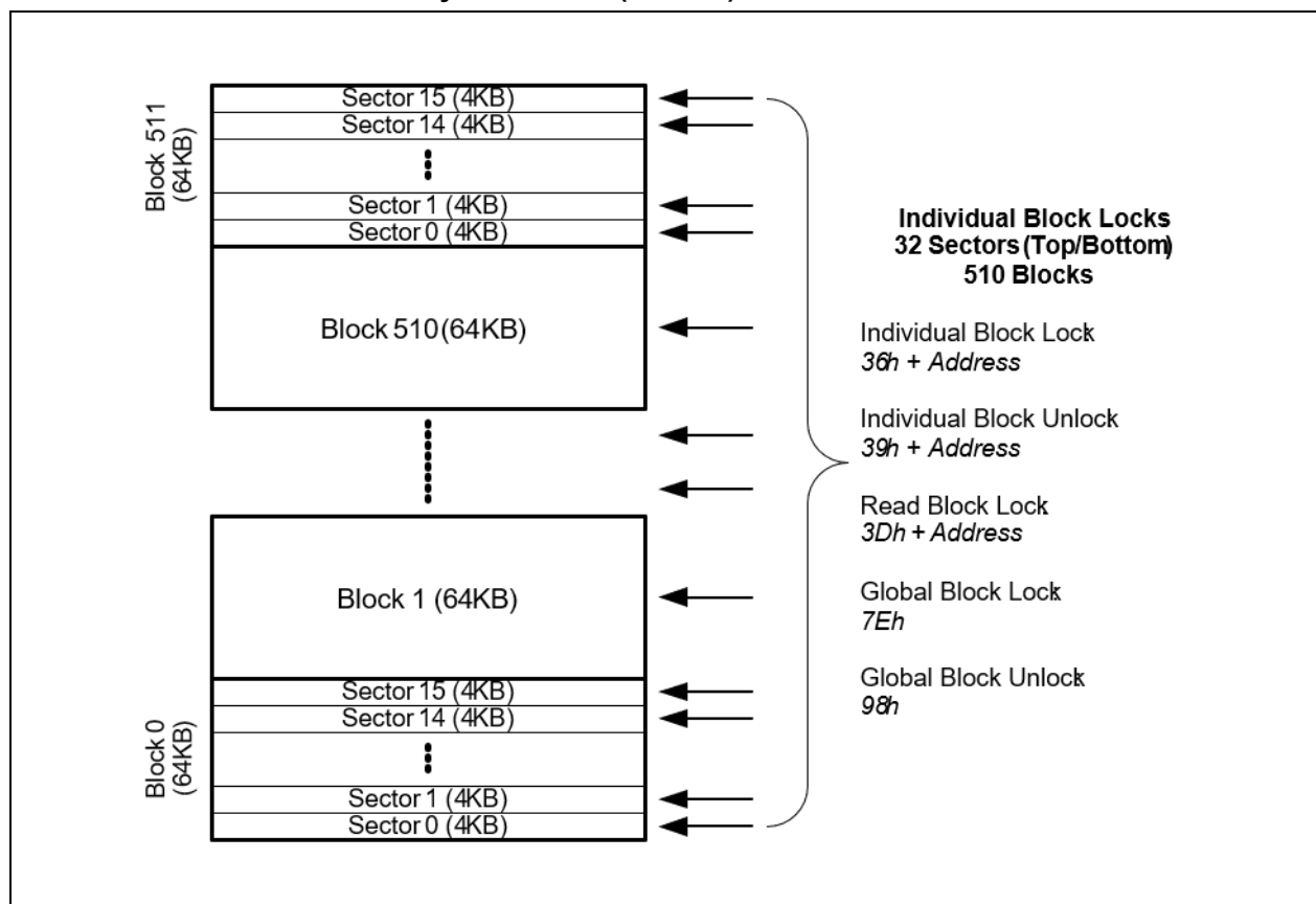
Figure 5-2. Individual Block/Sector Locks
