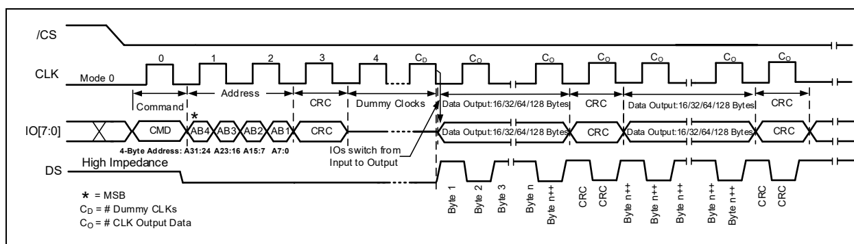
Figure 19-4g. CRC-In-Transit 8d-0-8d Read SFDP Command Protocol (ODDR Mode)
