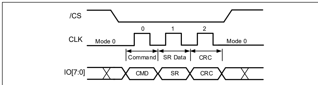
Figure 19-4b. 8d-0-8d Write Register CRC-In-Transit Command Protocol (ODDR Mode)
