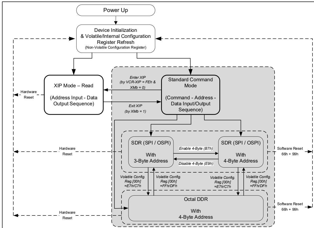
Figure 4-1. W35T25NW Serial Flash Memory Operation Diagram
