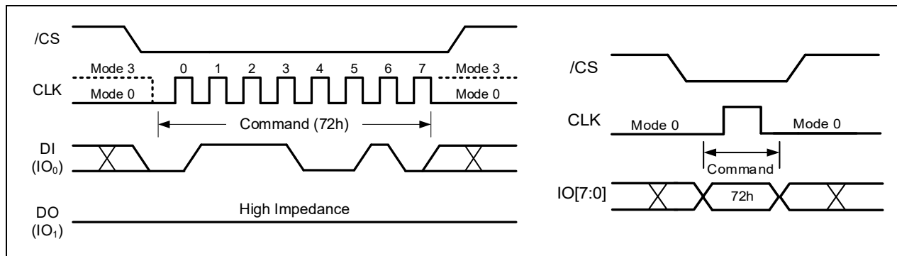
Figure 17-3. Reset ECC Counters for SDR Mode (left) or ODDR Mode (right)
