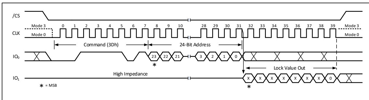
Figure 14-3a. Read Block/Sector Lock Command (SDR Mode)
