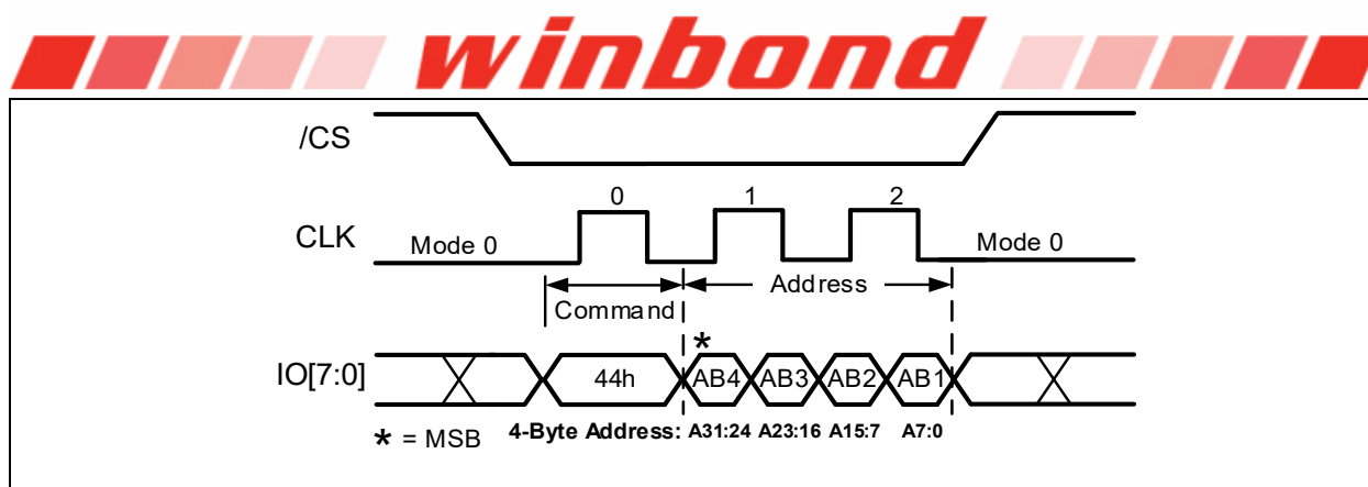
Figure 15-2b. Erase Security Registers Command (ODDR Mode) A 32-Bit Address is required when the device is operating in ODDR mode
