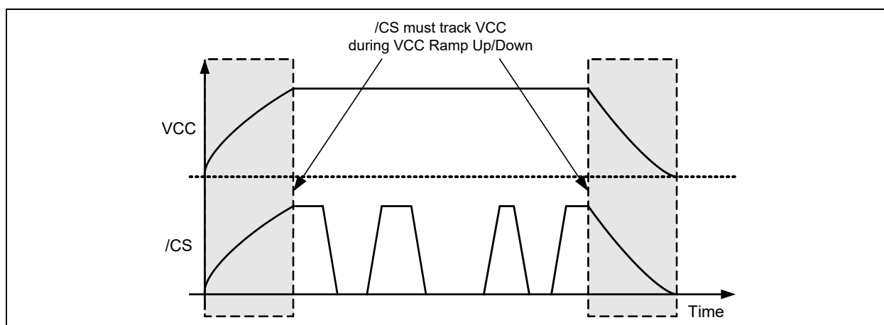
Figure 20-2. Power-up, Power-Down Requirement
