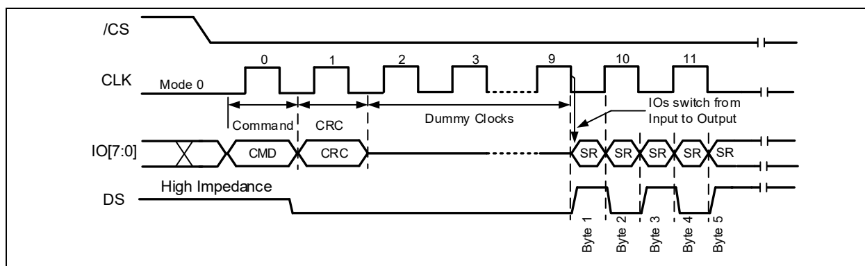
Figure 19-4d. 8d-0-8d Read Register CRC-In-Transit Command Protocol (ODDR Mode)
