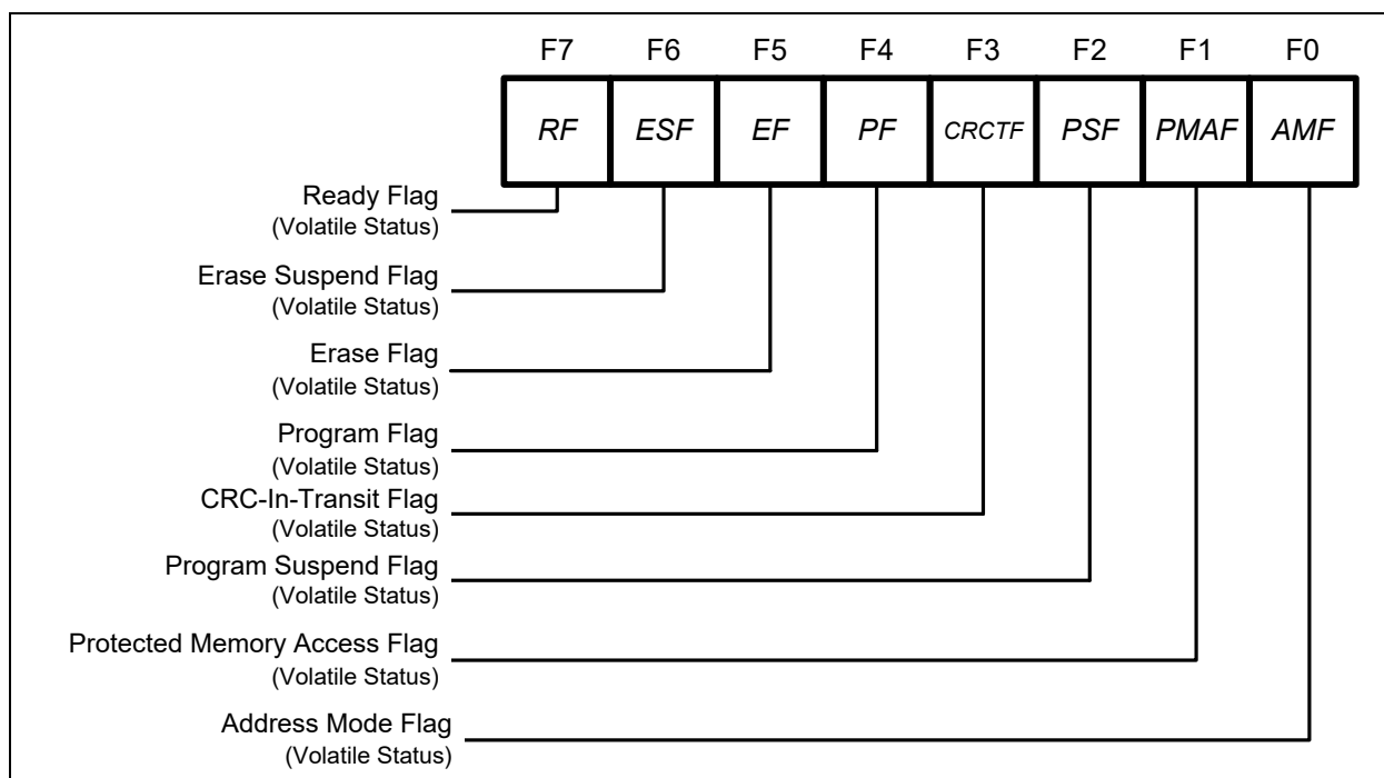
Figure 5-3. Flag Register
