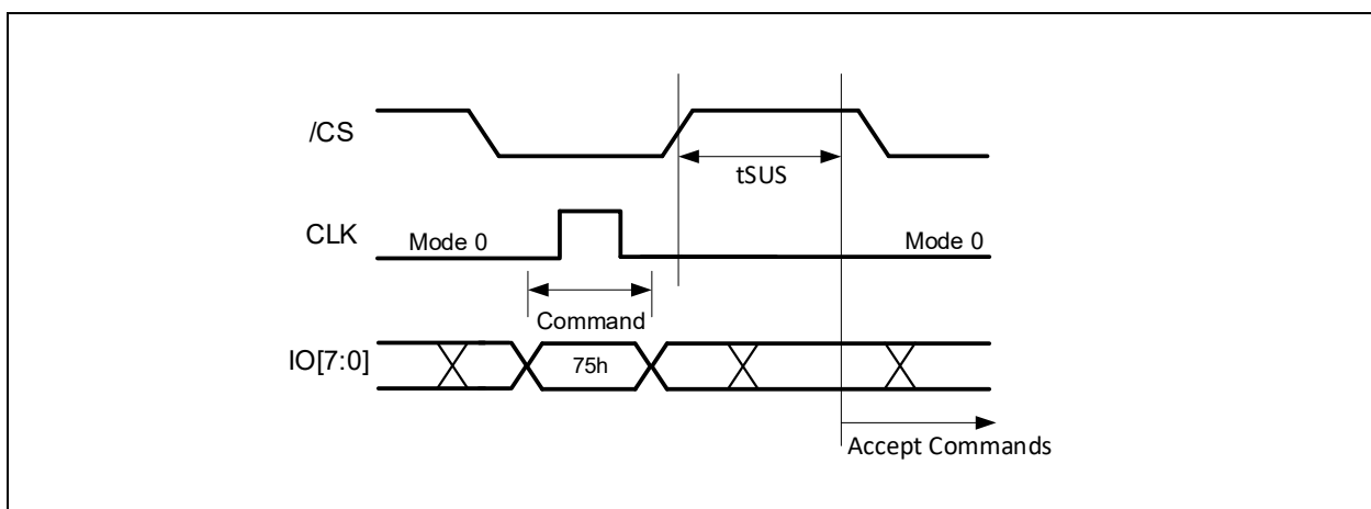
Figure 13-1b. Erase/Program Suspend Command (ODDR Mode)
