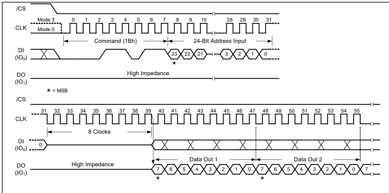
Figure 19-3a. Read 8-Byte CRC Code Command Sequence (1-1-1 SDR Mode)
