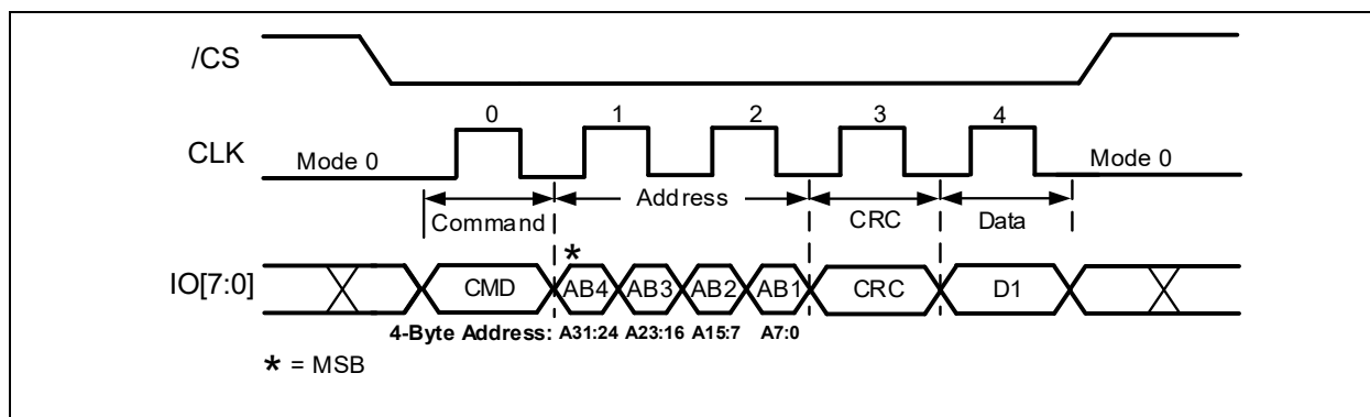
Figure 19-4c. 8d-8d-8d Write Register with Address CRC-In-Transit Command Protocol (ODDR Mode)
