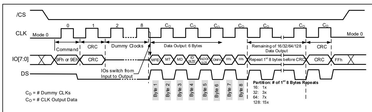
Figure 19-4f. 8d-0-8d Read ID CRC-In-Transit Command Protocol (ODDR Mode)
