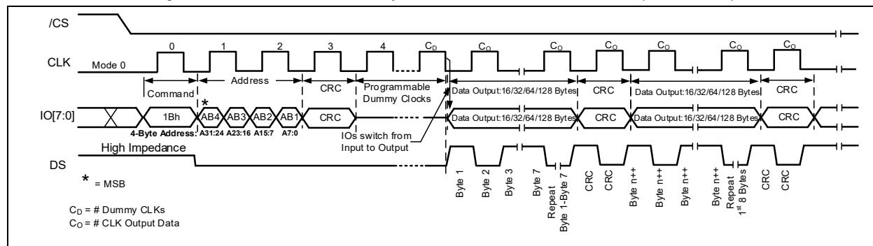
Figure 19-4m. 8d-8d-8d CRC-In-Transit Read 8-Byte CRC code Command Protocol (ODDR Mode)
