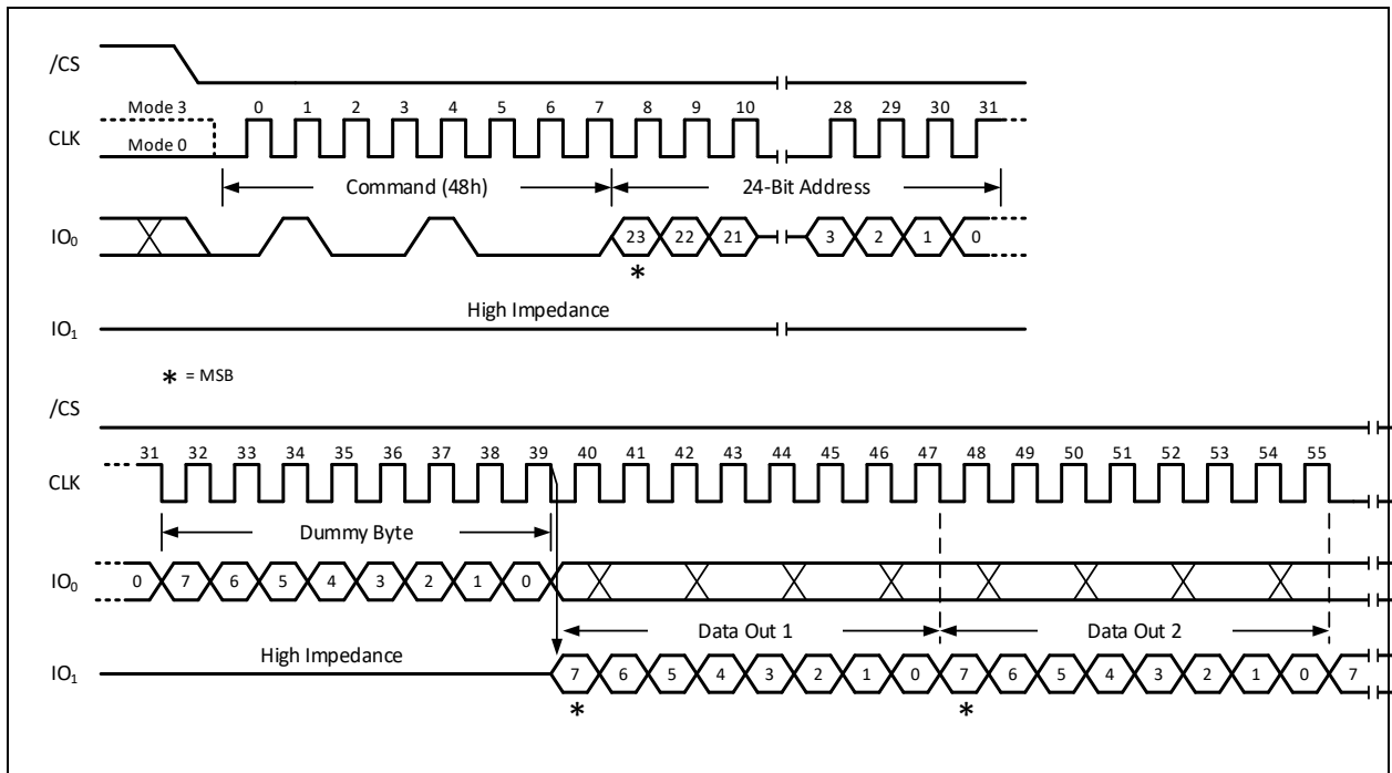
Figure 15-4a. Read Security Registers Command (SDR Mode)
