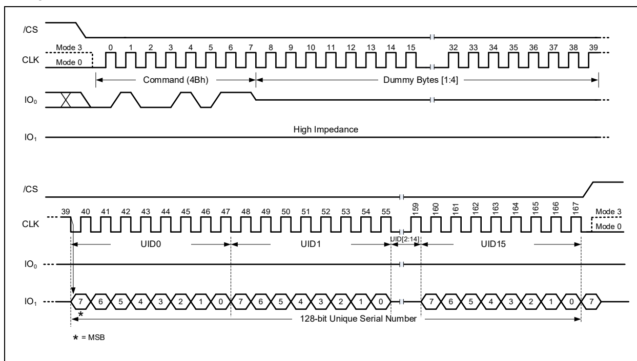
Figure 15-1a. Read Unique ID Command (SDR Mode)
