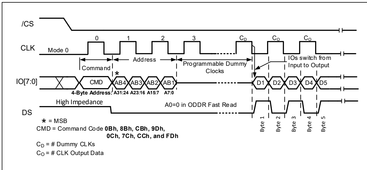
Figure 10-11. ODDR Fast Read Command (8d-8d-8d ODDR) A 32-Bit Address is required when the device is operating in ODDR Mode
