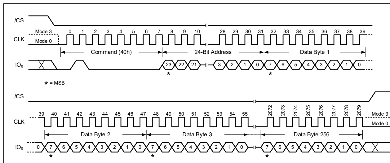
Figure 18-4. Program Tuning Data Pattern Command (1-1-1 SDR Mode) A 32-Bit Address is required when the device is operating in 4-Byte Address Mode
