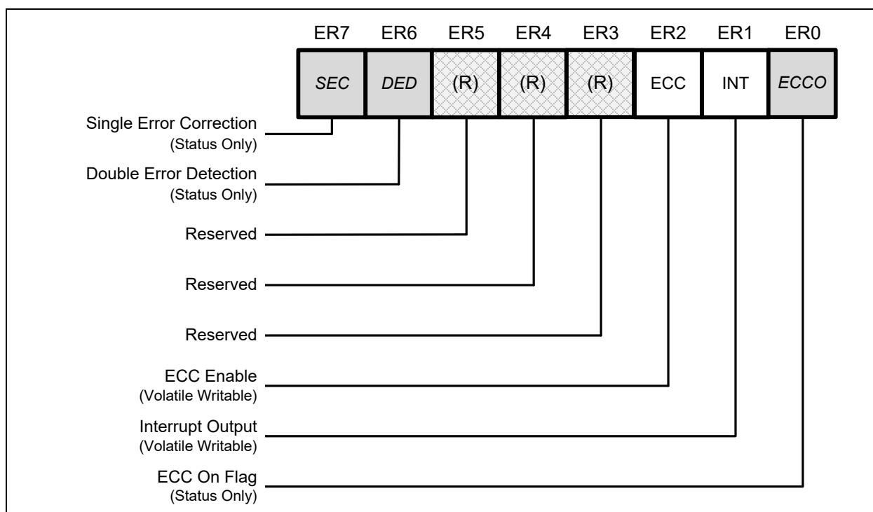
Figure 5-4. ECC Status Register
