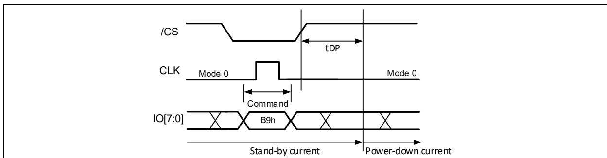
Figure 16-1b. Deep Power-down Command (ODDR Mode)
