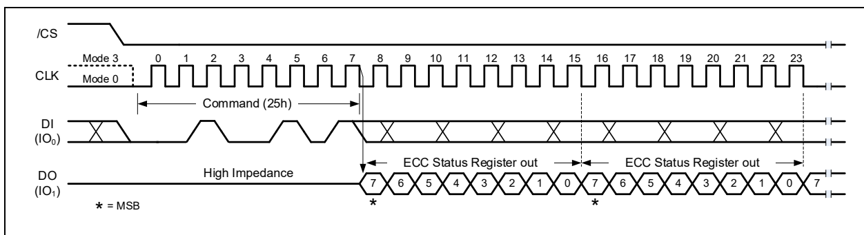
Figure 17-1a. Read ECC Status Register Command (SDR Mode)
