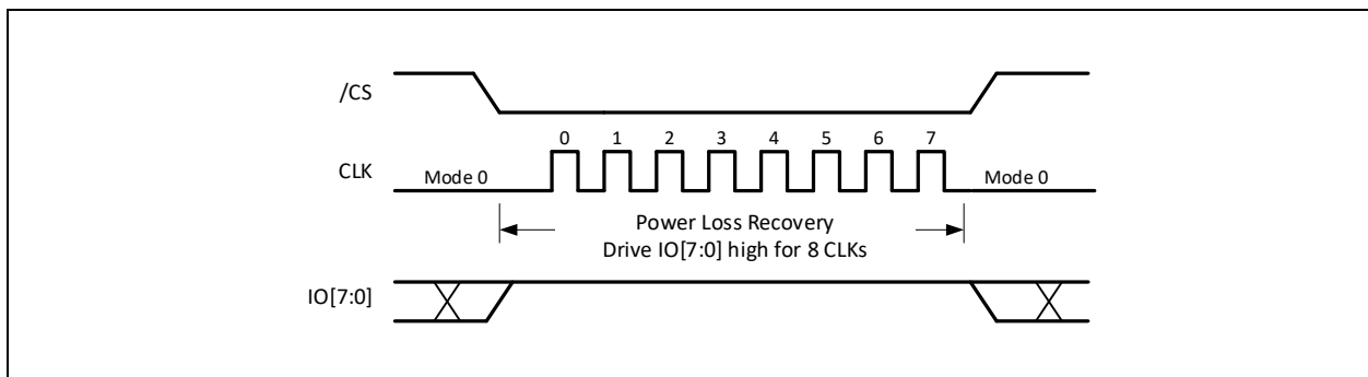
Figure 4-6. Power Loss Interface Recovery
