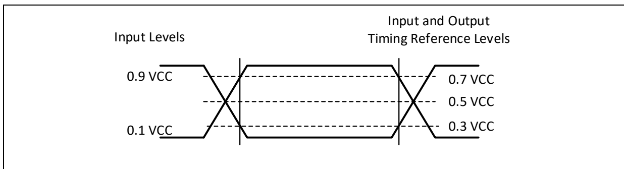
Figure 20-4. AC Measurement I/O Waveform
