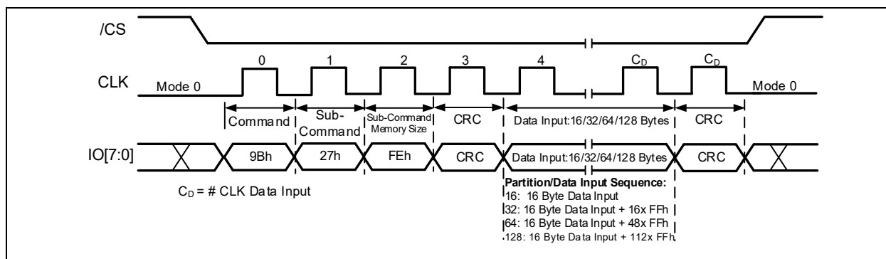
Figure 19-4j. CRC-In-Transit 8d-8d-8d CRC-At-Rest Memory Range Command Protocol (ODDR Mode)
