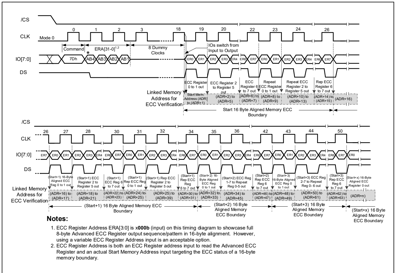
Figure 17-4b. Read Advanced ECC Status Register Command (ODDR Mode)
