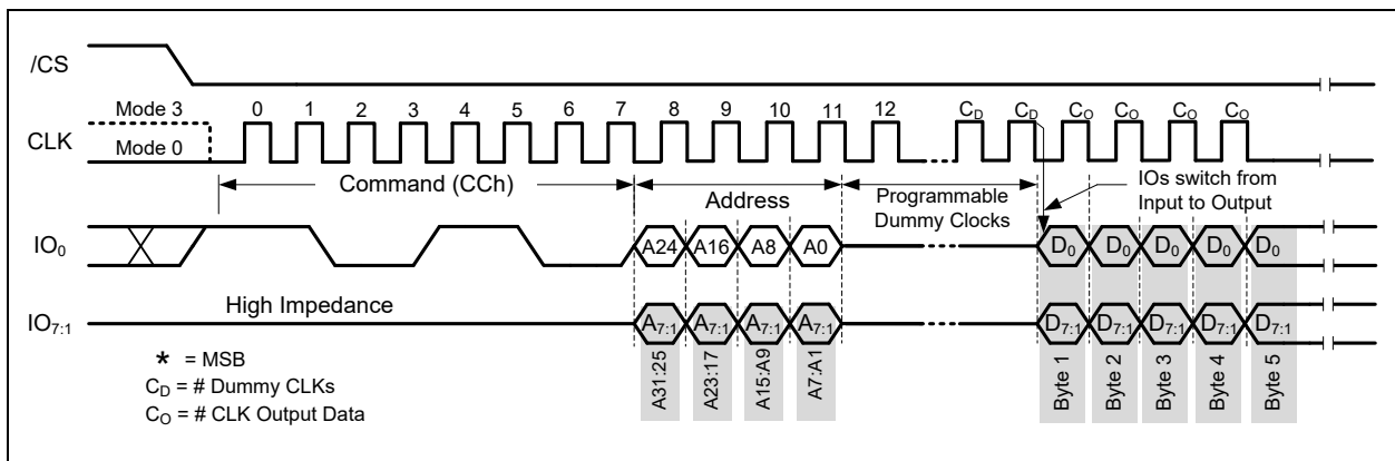
Figure 10-8. Fast Read Octal I/O Command with 4-Byte Address (1-8 SDR)
