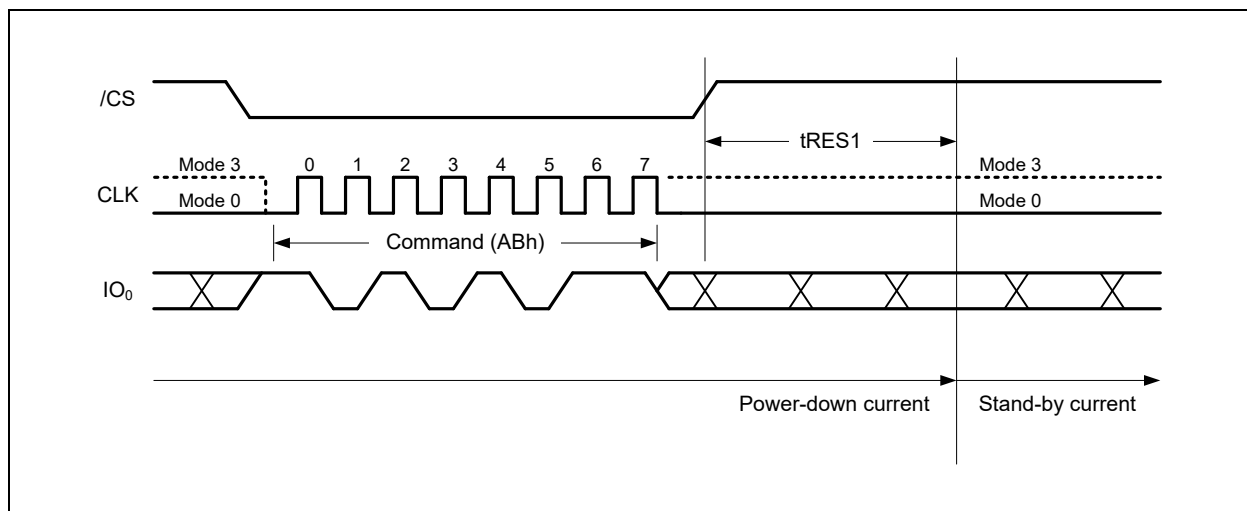
Figure 16-2a. Release Power-down Command (SDR Mode)
