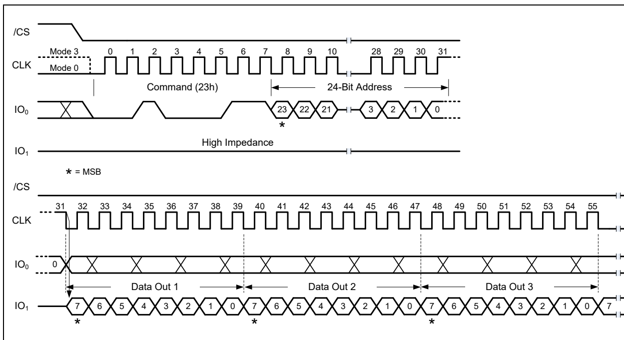
Figure 18-1. (1-1-1) Read DLP Command (1-1-1 SDR Mode)
