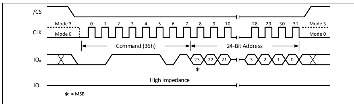
Figure 14-4a. Individual Block/Sector Lock Command (SDR Mode)
