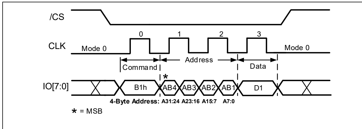
Figure 8-6b. Write Non-Volatile Configuration Command (ODDR Mode) A 32-Bit Address is required when the device is operating in ODDR mode
