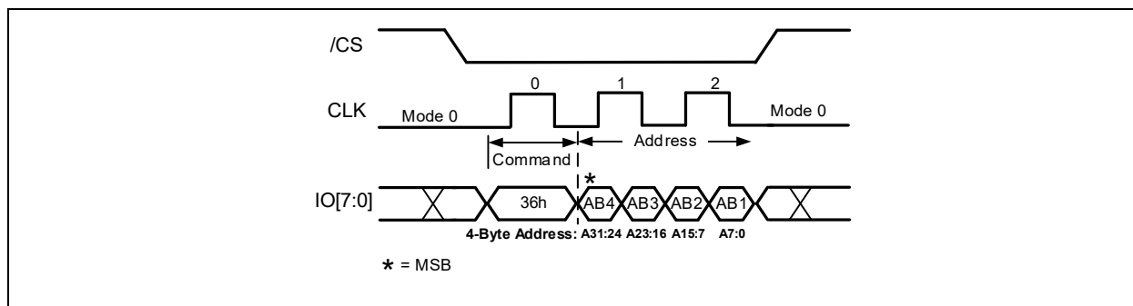
Figure 14-4b. Individual Block/Sector Lock Command (ODDR Mode)
