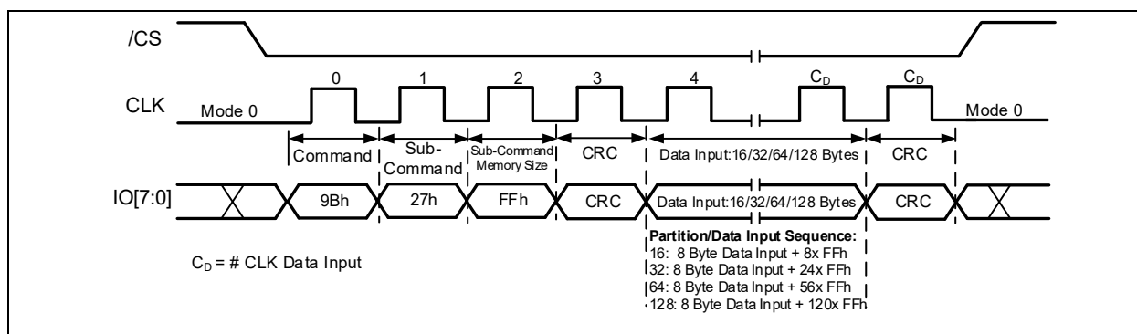
Figure 19-4i. CRC-In-Transit 8d-8d-8d CRC-At-Rest Full Memory Command Protocol (ODDR Mode)
