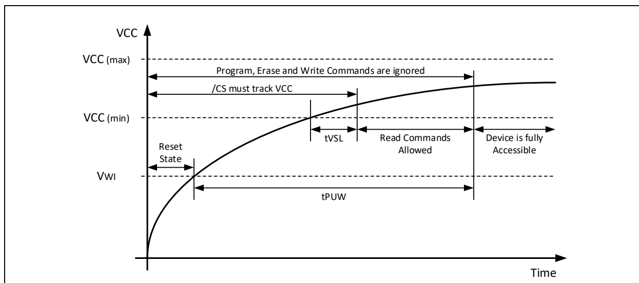
Figure 20-1. Power-up Timing and Voltage Levels
