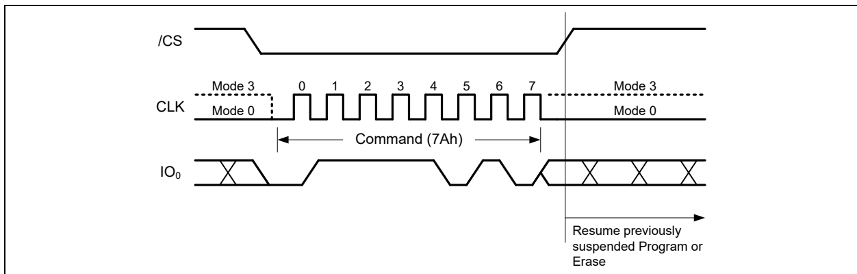
Figure 13-2a. Erase/Program Resume Command (SDR Mode)
