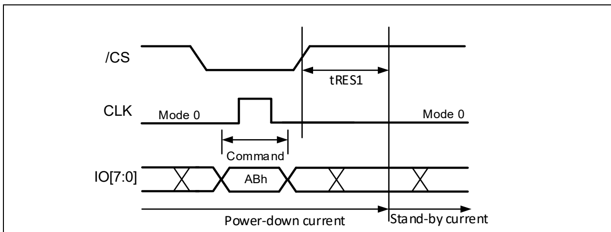
Figure 16-2b. Release Power-down Command (ODDR Mode)
