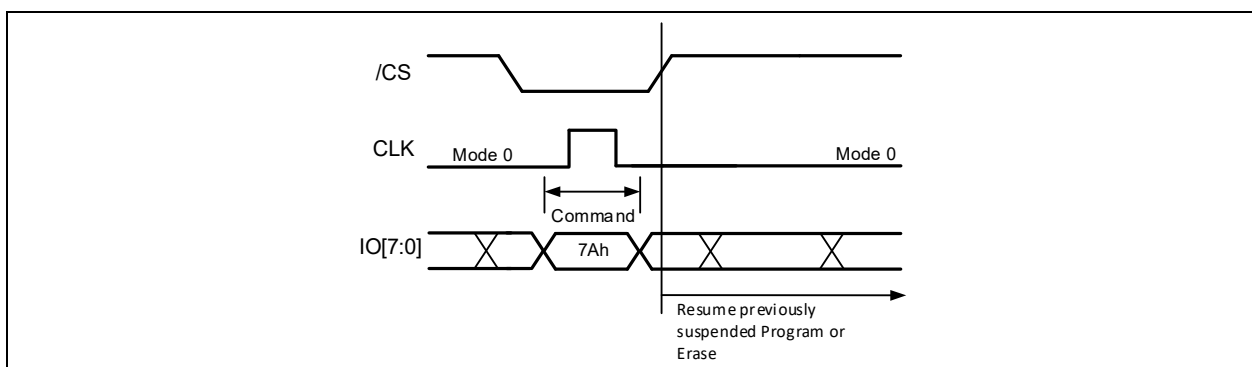
Figure 13-2b. Erase/Program Resume Command (ODDR Mode)
