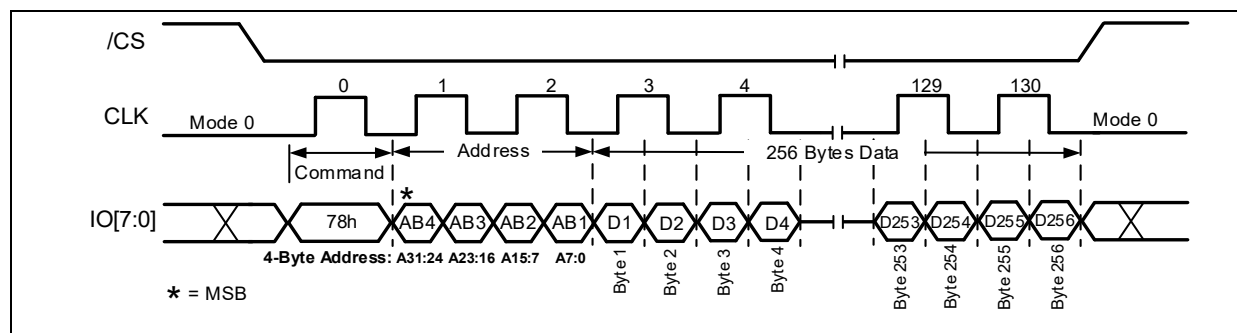
Figure 18-5b. (8d-8d-8d) Program DLP Register Command (8d-8d-8d ODDR Mode)
