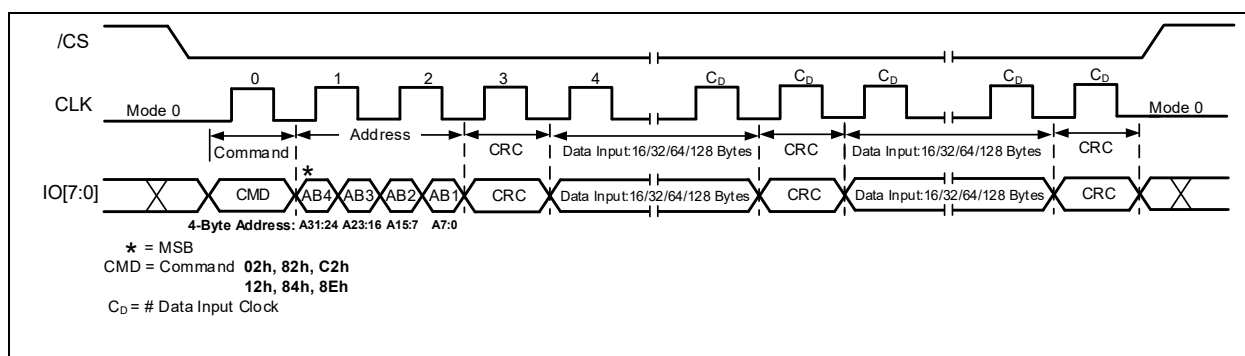
Figure 19-4h. CRC-In-Transit 8d-8d-8d Page Program Command Protocol (ODDR Mode)
