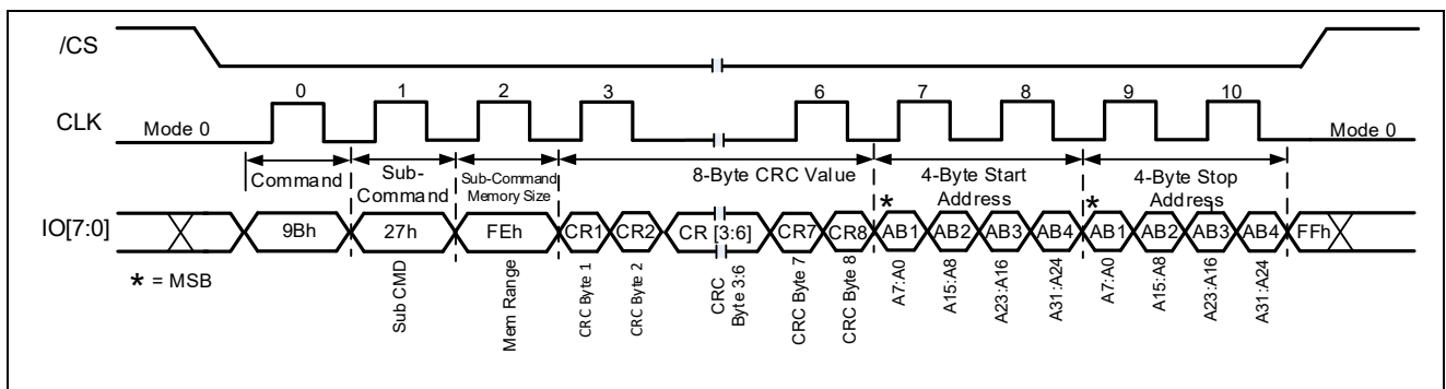
Figure 19-2b. ODDR CRC-At-Rest Memory Range Command Sequence (ODDR Mode)
