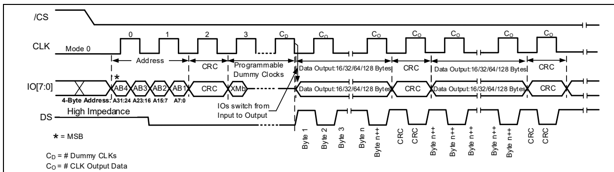
Figure 19-4o. 0-8d-8d XIP Read Memory CRC-In-Transit Command Protocol (ODDR Mode)
