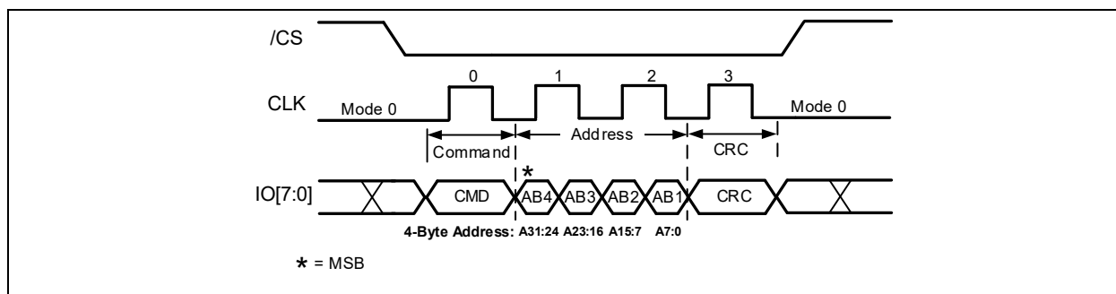
Figure 19-4k. CRC-In-Transit 8d-8d-0 Sector/Block Erase and Erase DLP Register Command Protocol (ODDR Mode)
