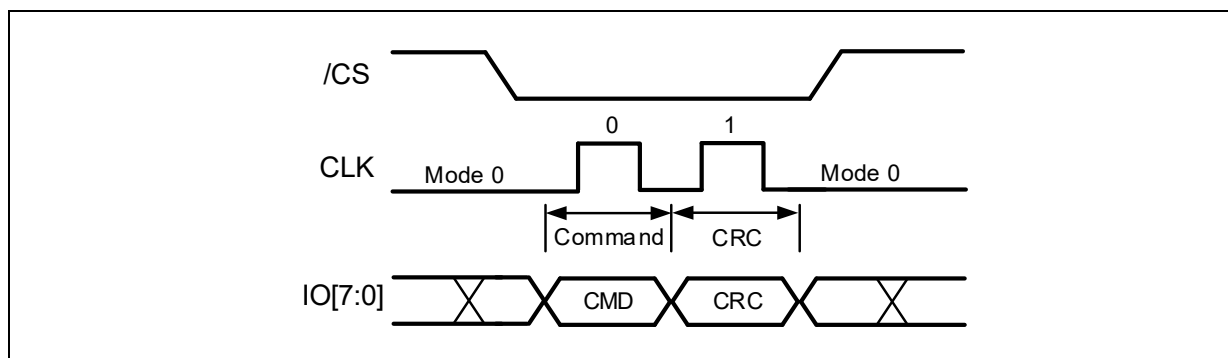
Figure 19-4a. 8d-0-0 CRC-In-Transit Command Protocol (ODDR Mode)
