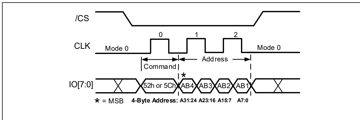
Figure 12-6. 32KB Block Erase Command (ODDR Mode)
