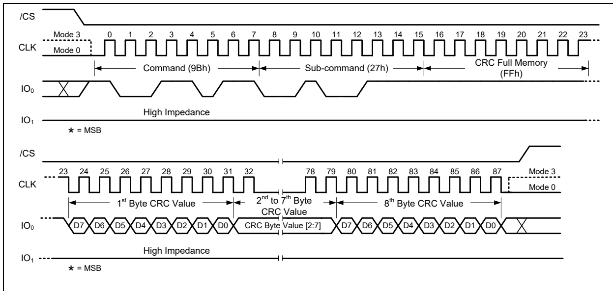
Figure 19-1a. CRC-At-Rest Full Memory Command Sequence (SDR Mode)
