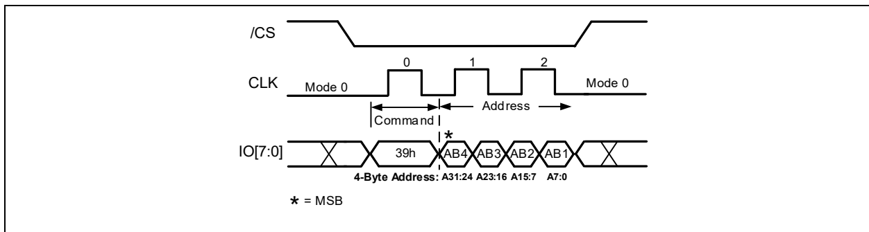
Figure 14-5b. Individual Block/Sector Unlock Command (ODDR Mode)
