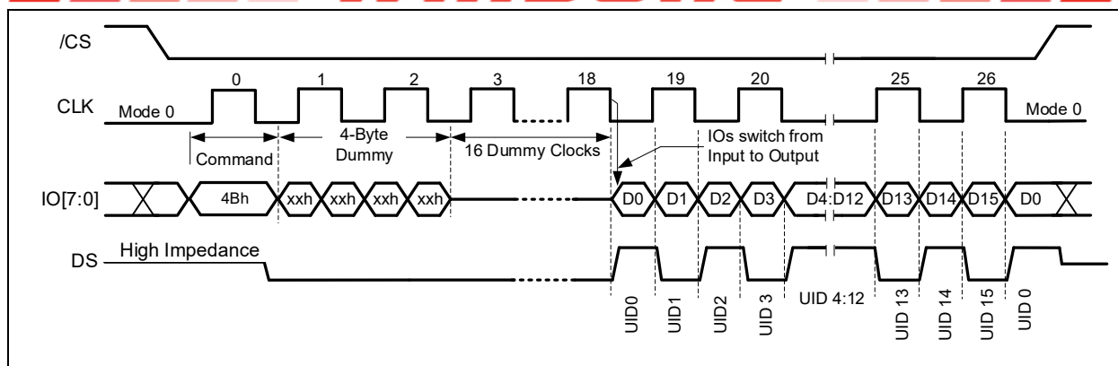
Figure 15-1b. Read Unique ID Command (ODOR Mode)
