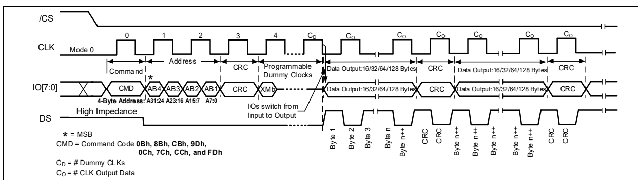
Figure 19-4n. 8d-8d-8d Read Memory with XIP Entry CRC-In-Transit Command Protocol (ODDR Mode)
