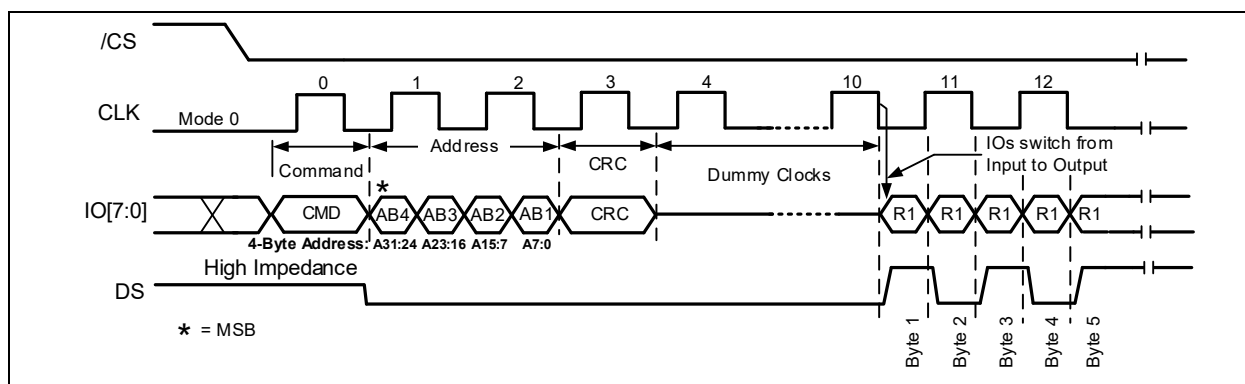
Figure 19-4e. 8d-8d-8d Read Register with Address CRC-In-Transit Command Protocol (ODDR Mode)
