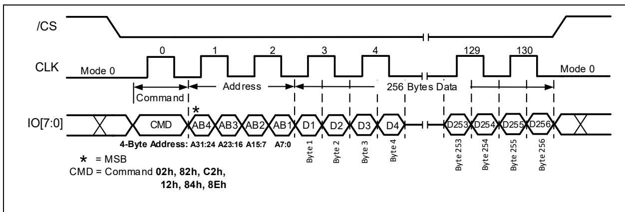
Figure 11-7. Octal DDR Page Program Commands (ODDR Mode) A 32-Bit Address is required when the device is operating in ODDR mode
