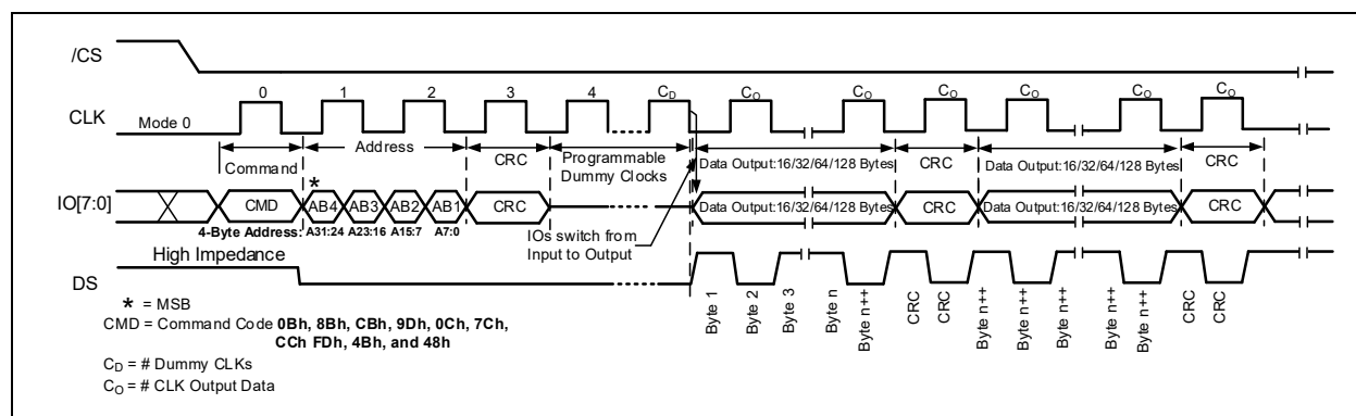
Figure 19-4l. 8d-8d-8d Read Memory CRC-In-Transit Command Protocol (ODDR Mode)
