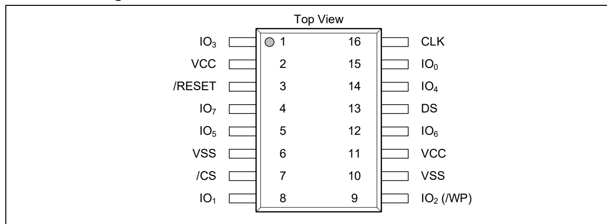
Figure 3-1. W35T25NW Industrial Grade Pin Assignments, 16-pin SOIC 300-mil (Package Code SF)
