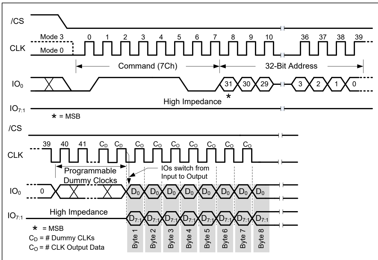
Figure 10-6. Fast Read Octal Output with 4-Byte Address Command (1-1-8 SDR Mode)
