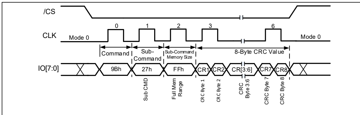
Figure 19-1b. ODDR CRC-At-Rest Full Memory Command Sequence (ODDR Mode)
