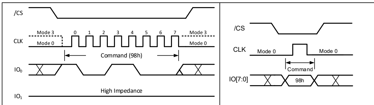
Figure 14-2. Global Block/Sector Unlock Command for SDR Mode (left) or ODDR Mode (right)
