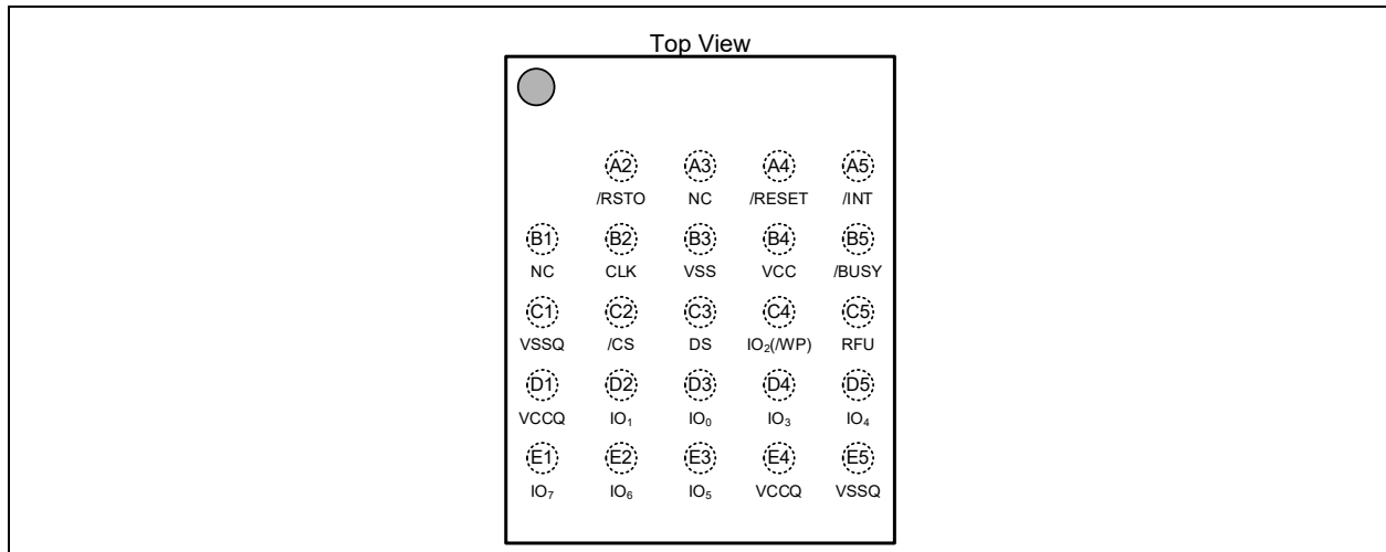
Figure 3-2. W35T25NW Ball Assignments, 24-ball (5x5 ball array) TFBGA 6x8-mm (Package Code TB)
