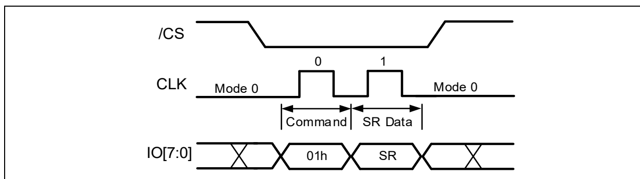
Figure 8-4b. Write Status Register Command (ODDR Mode)
