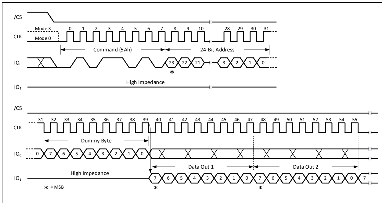
Figure 7-2a. Read SFDP Register Command Sequence (SDR Mode) A 24-Bit Address input only even when device is operating in 4-Byte Address Mode
