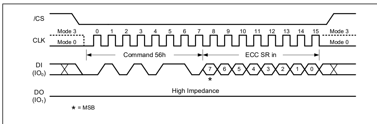
Figure 17-2a. Write ECC Status Register Command (SDR Mode)
