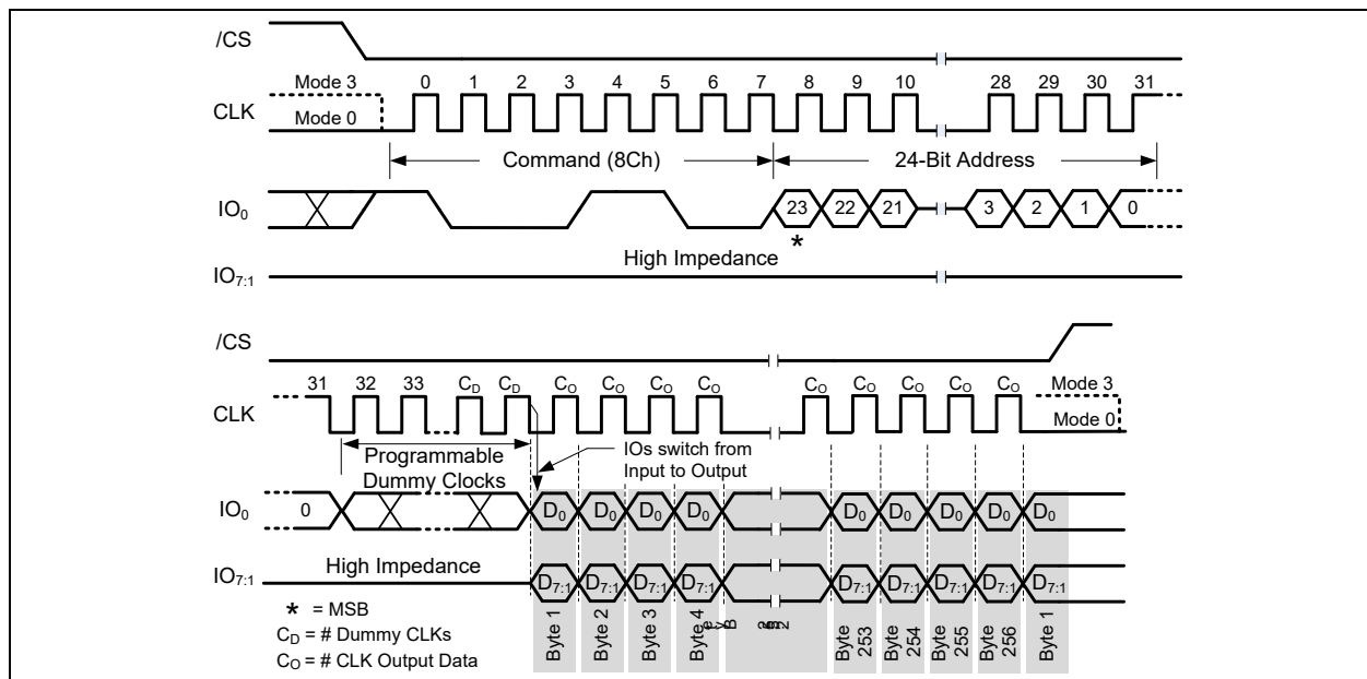
Figure 18-2. (1-1-8) Read DLP Command (1-1-8 SDR Mode)
