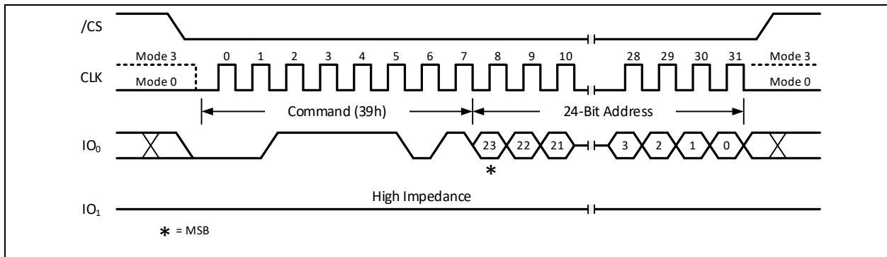
Figure 14-5a. Individual Block/Sector Unlock Command (SDR Mode)
