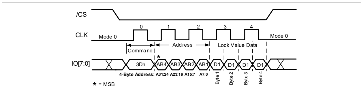
Figure 14-3b. Read Block/Sector Lock Command (ODDR Mode)
