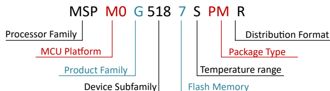
Figure 10-1. Device Nomenclature
