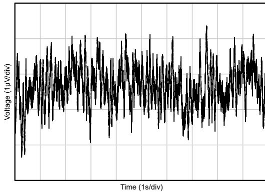
Figure 5-23. 0.1Hz to 10Hz Voltage Noise in Time Domain
