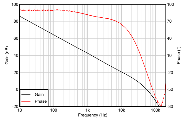
Figure 5-10. Open-Loop Gain and Phase vs Frequency
