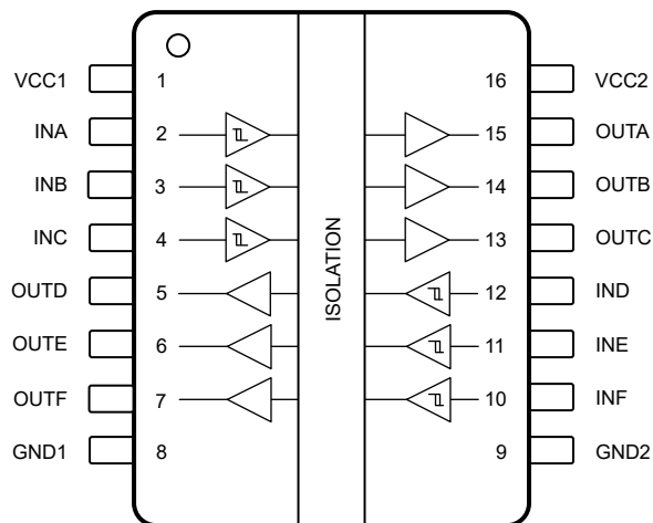
Figure 5-4. ISO6463 and ISO6463F Top View
