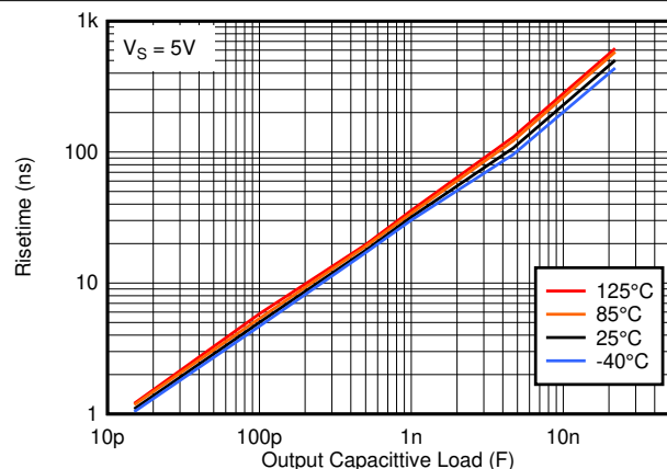
Figure 5-15. Risetime vs Capacitive Load
