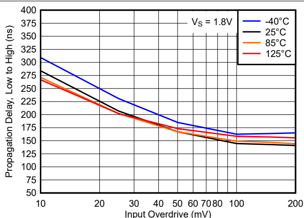
Figure 5-18. Propagation Delay, Low to High, 1.8V
