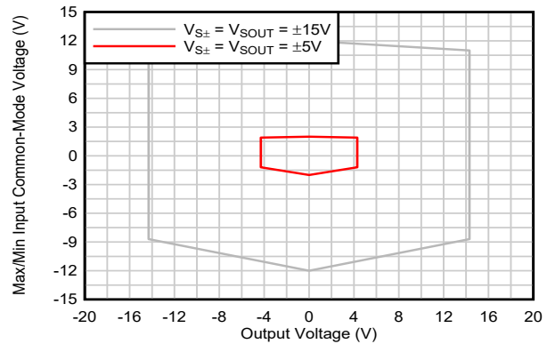
Figure 8-4. Input Common-Mode Voltage vs Output Voltage
