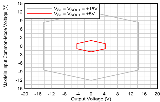
Figure 8-3. Input Common-Mode Voltage vs Output Voltage
