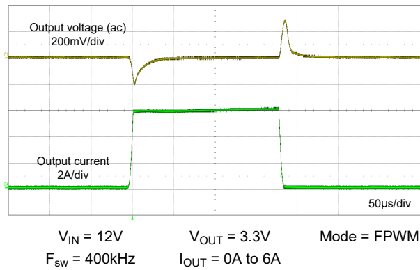
Figure 8-22. Load Transient
