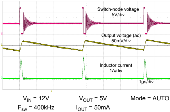
Figure 8-26. Steady-State Switching Waveform and Output Voltage Ripple
