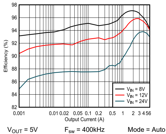
Figure 8-4. Efficiency - Auto Mode
