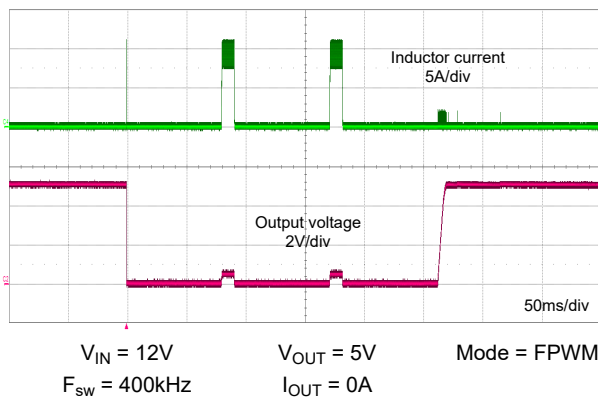
Figure 8-30. Short-Circuit Behavior
