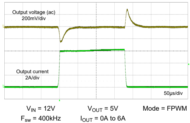
Figure 8-23. Load Transient
