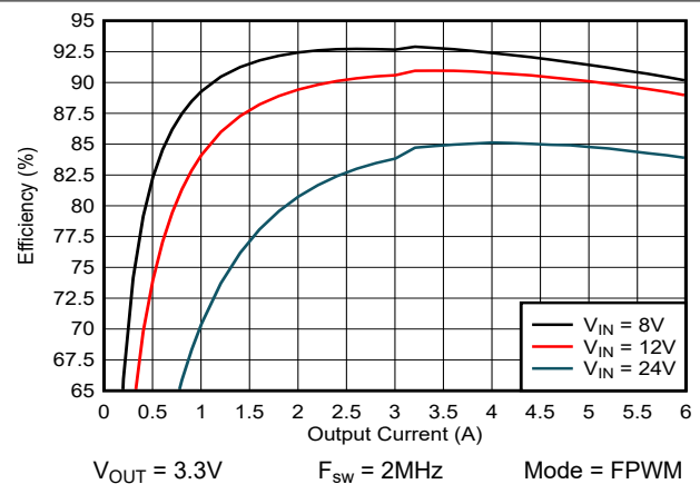
Figure 8-7. Efficiency - FPWM Mode
