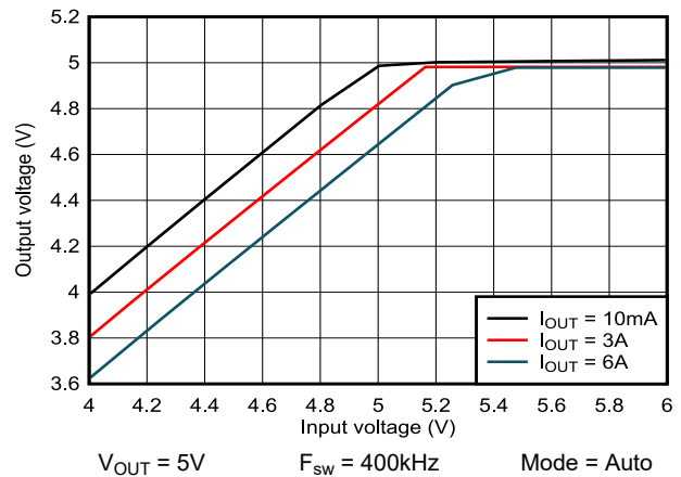
Figure 8-19. Dropout Curve
