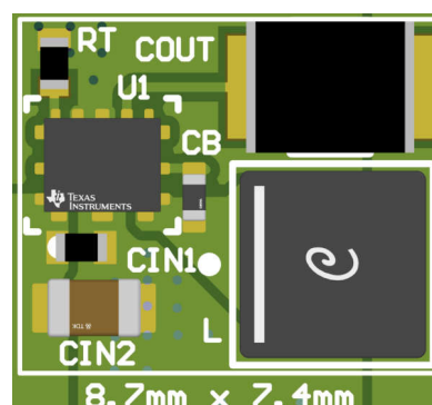
Figure 8-38. Ultra-Compact Fixed Output Voltage Configuration EVM Layout
