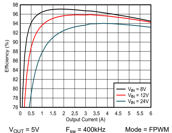
Figure 8-5. Efficiency - FPWM Mode
