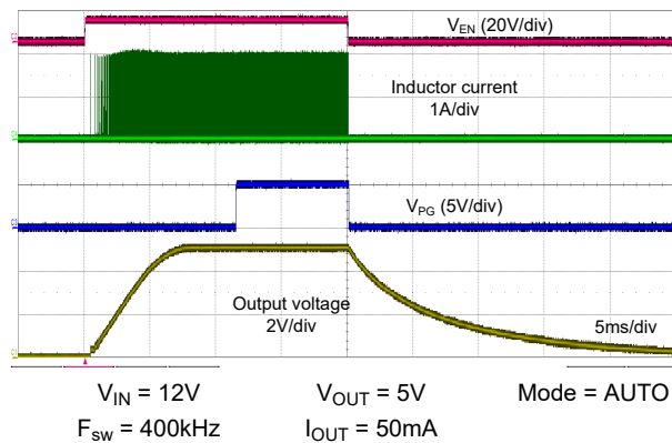
Figure 8-28. Enable Start-Up and Shutdown With 50mA Load
