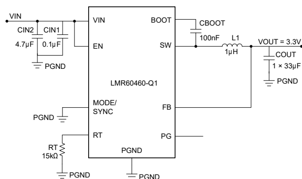
Figure 8-37. Fixed Output Version Schematic - 2.2MHz 3.3V
