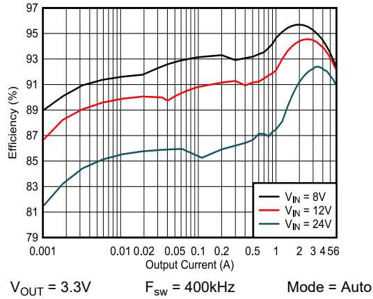
Figure 8-2. Efficiency - Auto Mode
