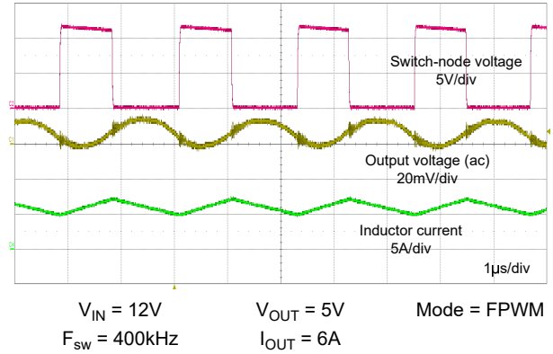
Figure 8-27. Steady-State Switching Waveform and Output Voltage Ripple
