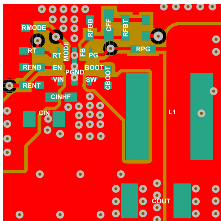
Figure 8-36. Adjustable Output Version
