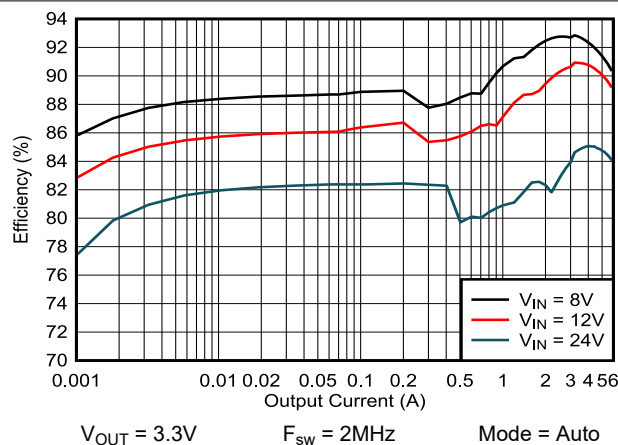
Figure 8-6. Efficiency - Auto Mode
