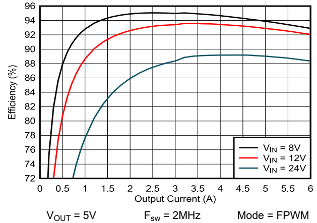
Figure 8-9. Efficiency - FPWM Mode
