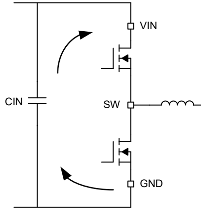
Figure 8-35. Current Loops With Fast Edges
