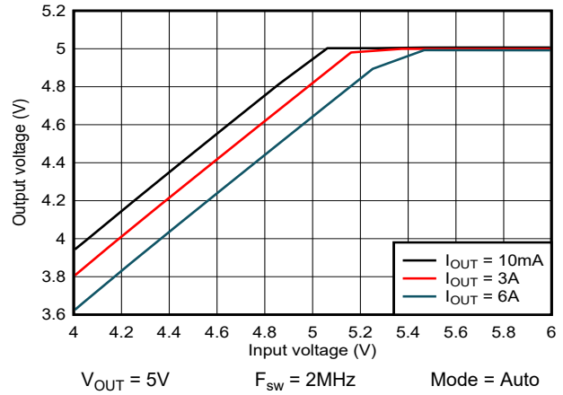
Figure 8-21. Dropout Curve
