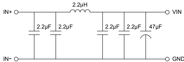
Figure 8-34. Recommended input EMI filter
