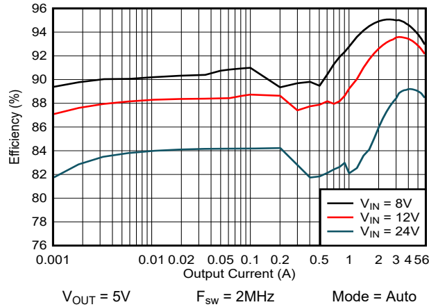
Figure 8-8. Efficiency - Auto Mode
