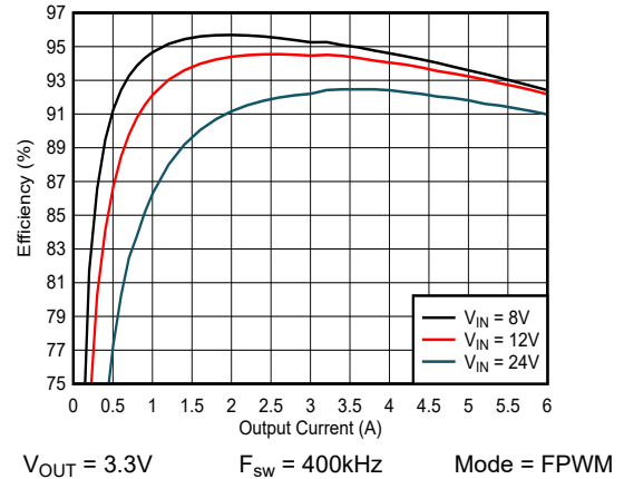
Figure 8-3. Efficiency - FPWM Mode
