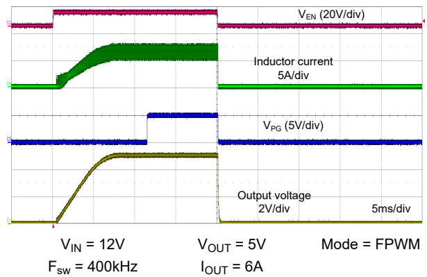
Figure 8-29. Enable Start-Up and Shutdown With 6A Load
