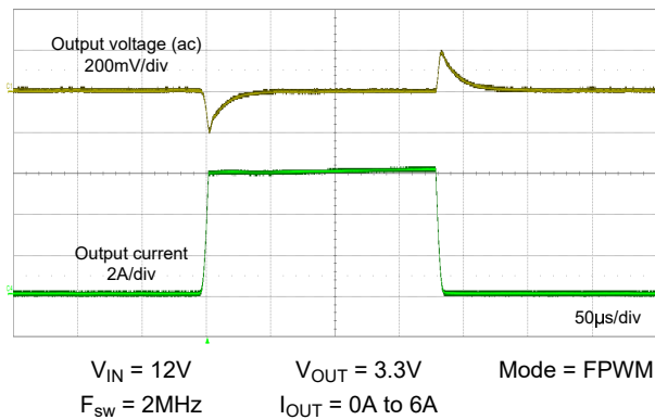
Figure 8-24. Load Transient
