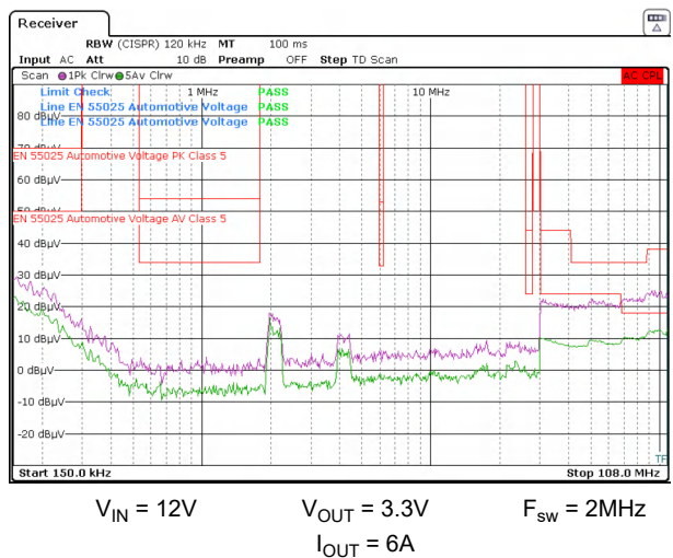
Figure 8-31. Conducted EMI vs CISPR 25 Limits (Pink: Peak Signal, Green: Average Signal)
