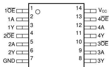
Figure 4-2. SN74AC125, PW Package (Top View)
