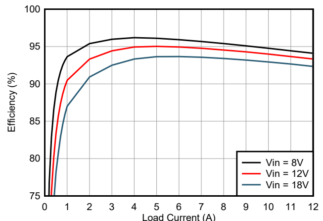
Typical Efficiency, V_{\text{OUT}} = 3.3\text{V} , F_{\text{SW}} = 440\text{kHz}
