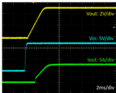
V_{IN} step to 12V 8A resistive load
