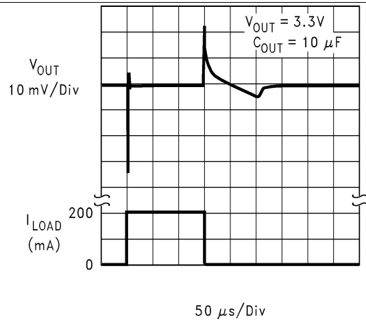
Figure 26. Load Transient Response
