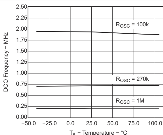
Figure 8-21. DCO Frequency vs Temperature (V CC = 3 V)
