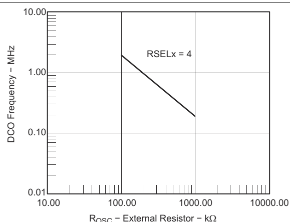
Figure 8-20. DCO Frequency vs R OSC (V CC = 3 V, T A = 25°C)
