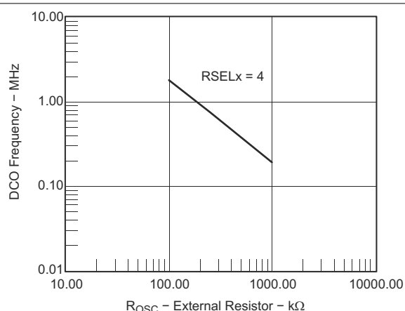
Figure 8-19. DCO Frequency vs R OSC (V CC = 2.2 V, T A = 25°C)
