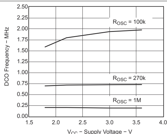
Figure 8-22. DCO Frequency vs Supply Voltage (T A = 25°C)
