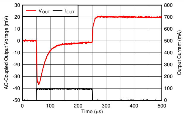
Figure 6-56. Load Transient
