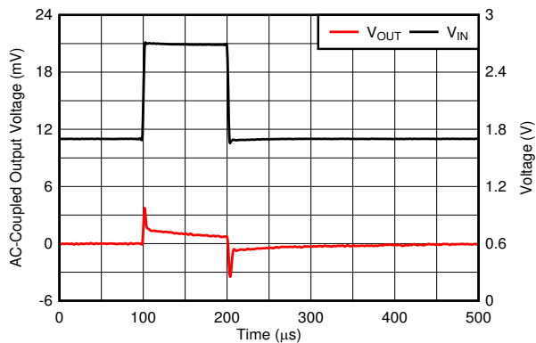
Figure 6-25. Line Transient
