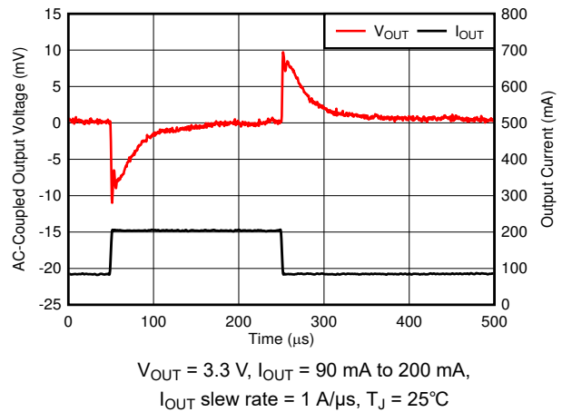
Figure 6-62. Load Transient
