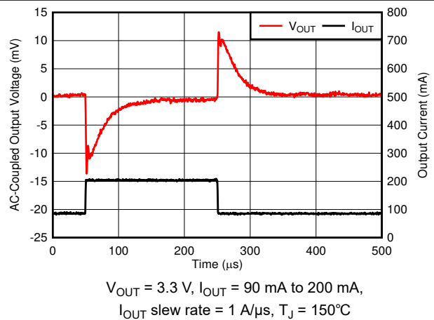
Figure 6-64. Load Transient
