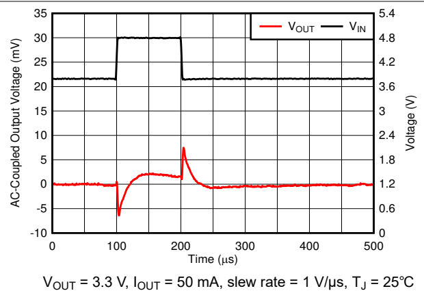
Figure 6-35. Line Transient
