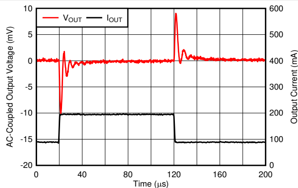
Figure 6-55. Load Transient
