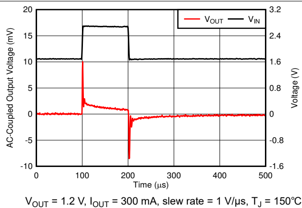
Figure 6-34. Line Transient
