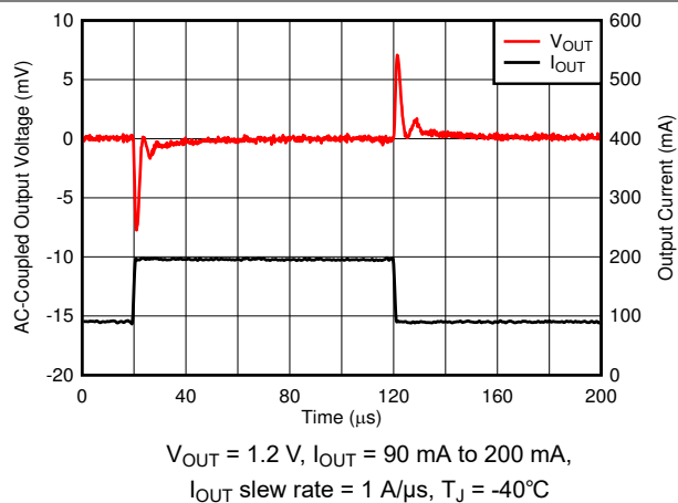
Figure 6-54. Load Transient
