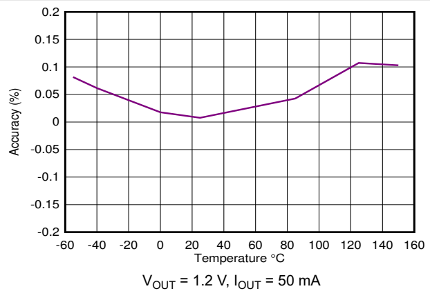
Figure 6-8. Accuracy vs Temperature
