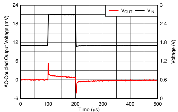
Figure 6-28. Line Transient
