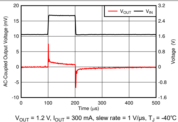
Figure 6-33. Line Transient
