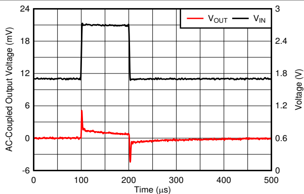
Figure 6-27. Line Transient
