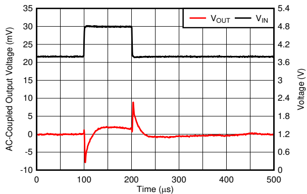
Figure 6-37. Line Transient
