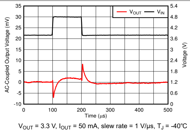
Figure 6-36. Line Transient
