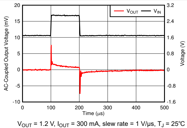
Figure 6-32. Line Transient
