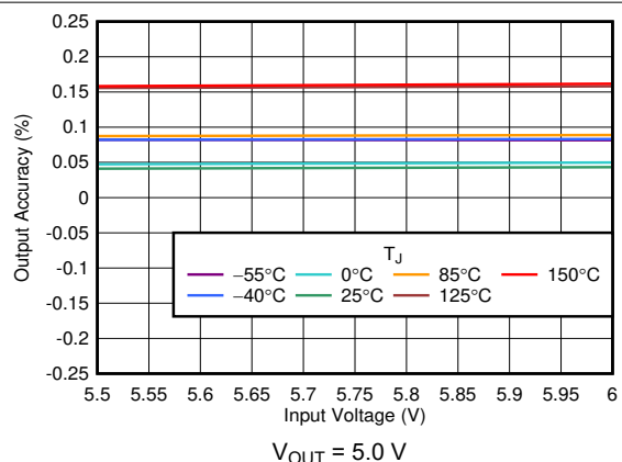
Figure 6-6. Output Accuracy vs V_{IN}
