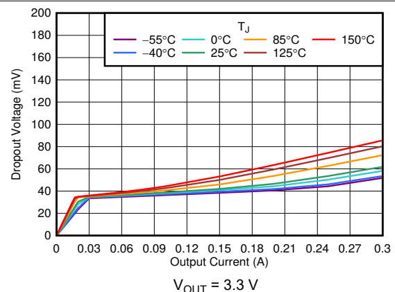
Figure 6-12. Dropout Voltage vs I_{\text{OUT}}
