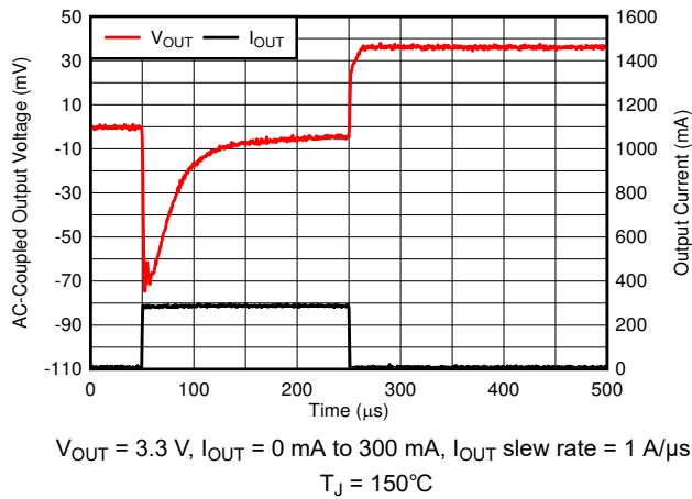
Figure 6-61. Load Transient
