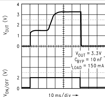
Figure 7-28. Turn-On Time (Legacy Chip)
