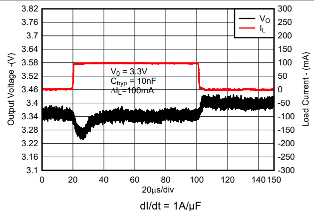
Figure 7-9. Load Transient Response (New Chip)
