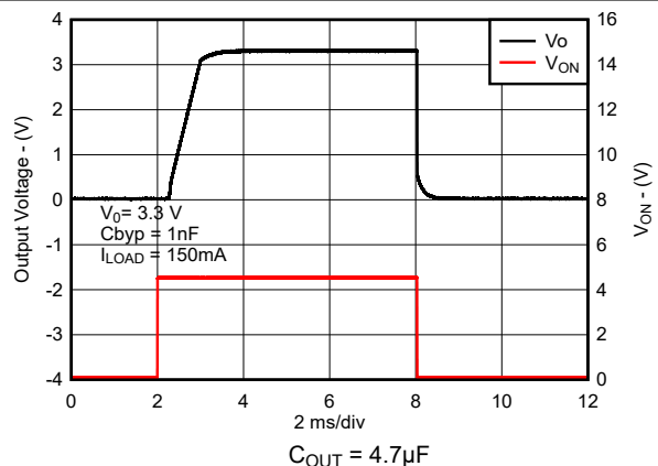
Figure 7-27. Turn-On Time (New Chip)
