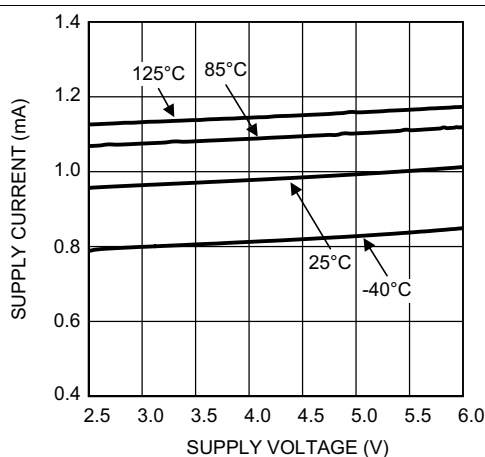
Figure 11. Supply Current vs Supply Voltage Quad LMV834
