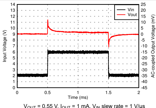
Figure 6-30. 0.55-V Line Transient
