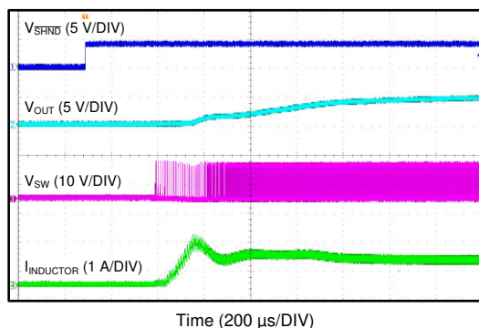
Figure 7-6. Start-Up Waveform ( V_{IN} = 12\text{ V} , V_{OUT} = 5\text{ V} , I_{Load} = 800\text{ mA} )
