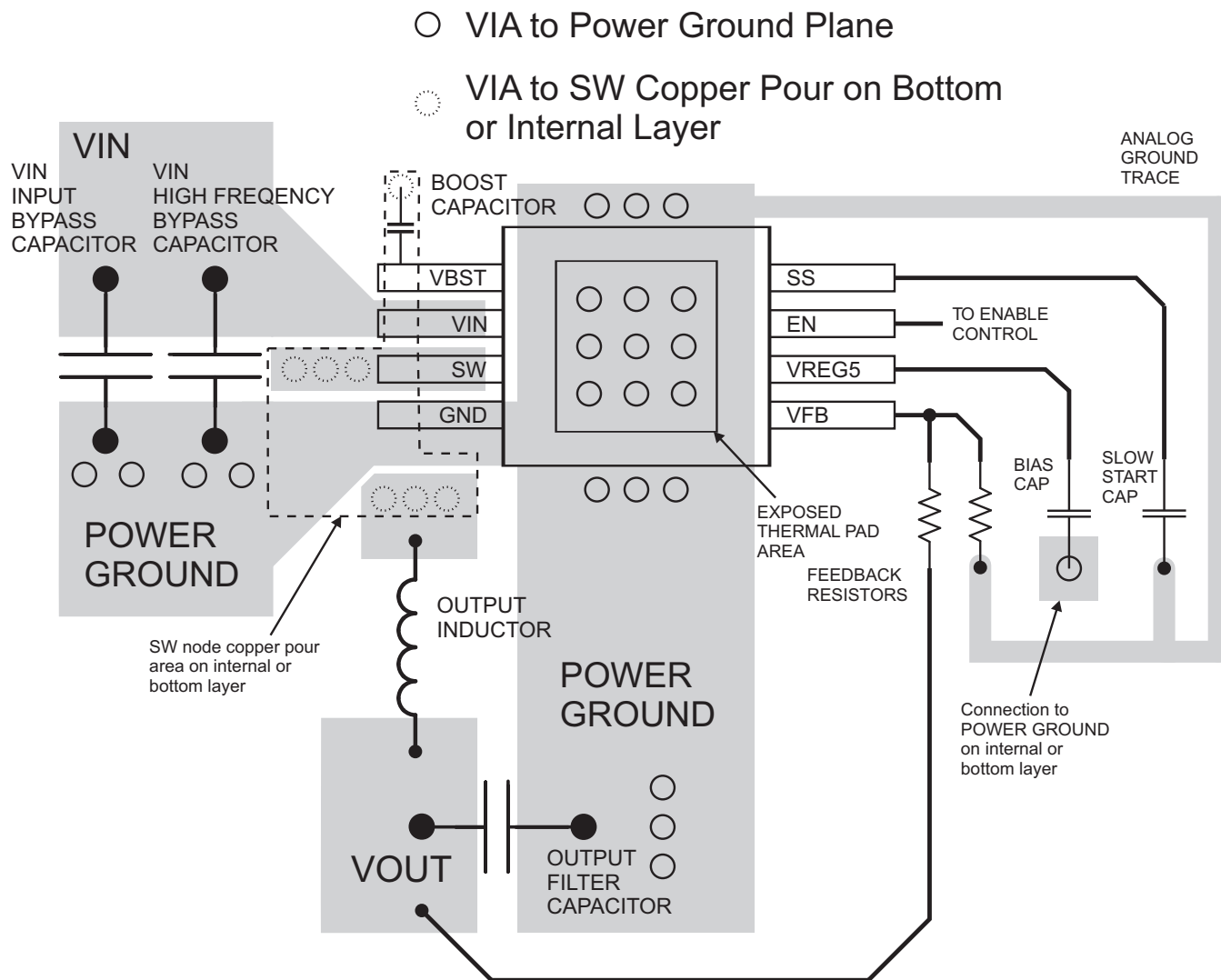
Figure 17. PCB Layout
