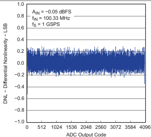
Figure 10. Differential Nonlinearity
