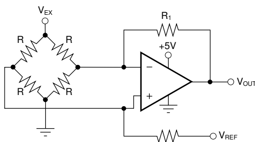
Figure 9-4. Bridge Amplifier
