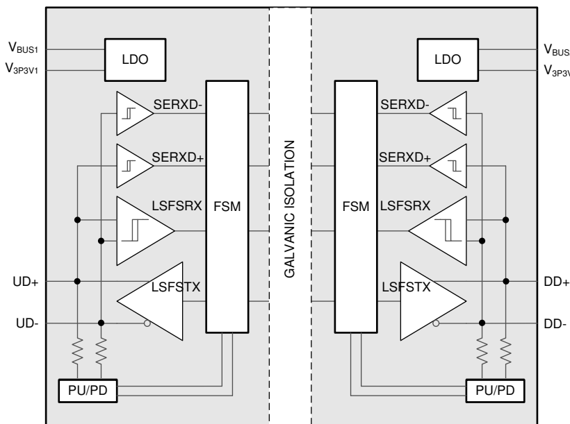
Figure 7-1. ISOUSB111 Simplified Functional Block Diagram
