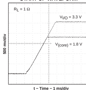
START-UP WAVEFORM
