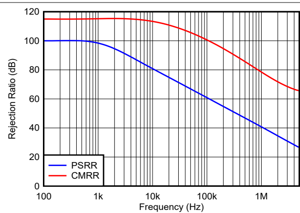
Figure 6-2. Power-Supply and Common-Mode Rejection Ratio
