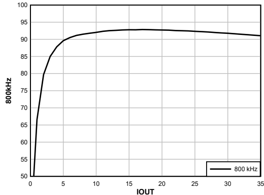
Figure 8-8. Efficiency, FCCM, Internal LDO
