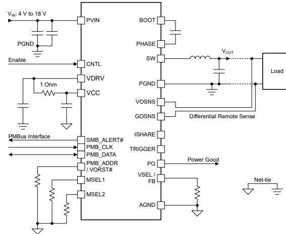
Simplified Schematic
