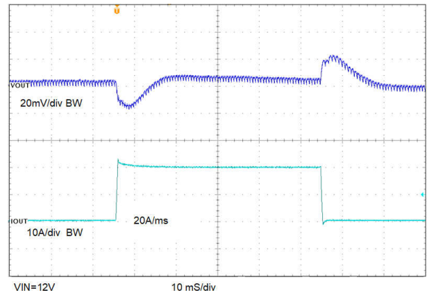
Figure 8-15. Load Transient 0A to 20A
