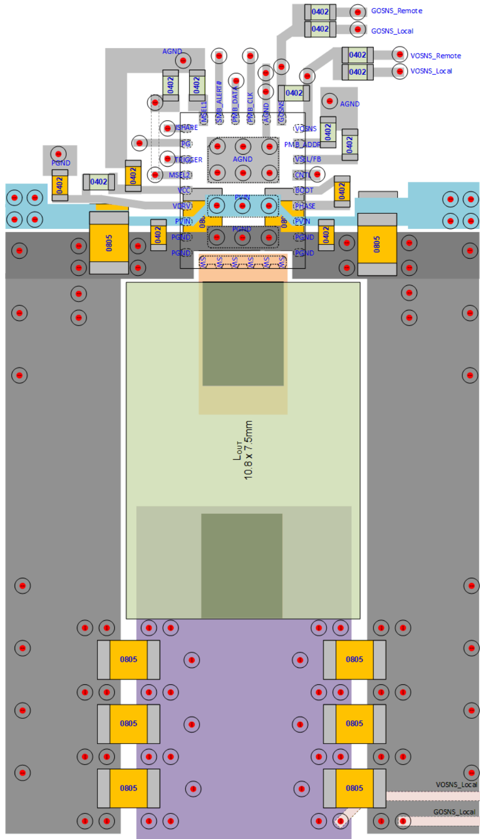
Figure 8-18. Layout Recommendation
