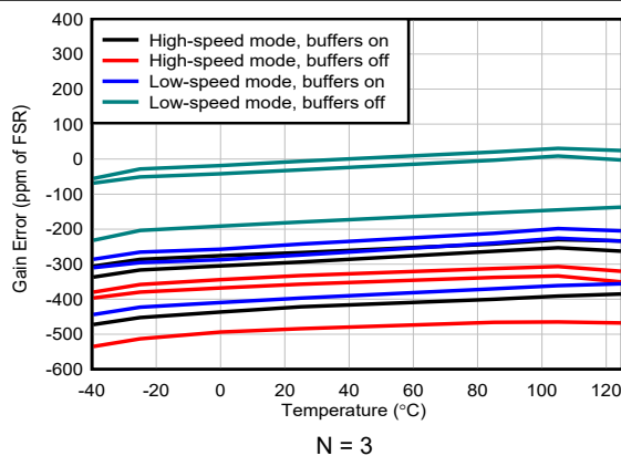
Figure 6-32. Gain Error vs Temperature
