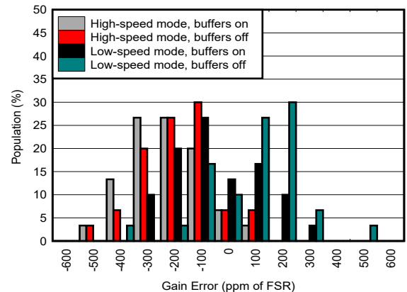
Figure 6-31. Gain Error Distribution
