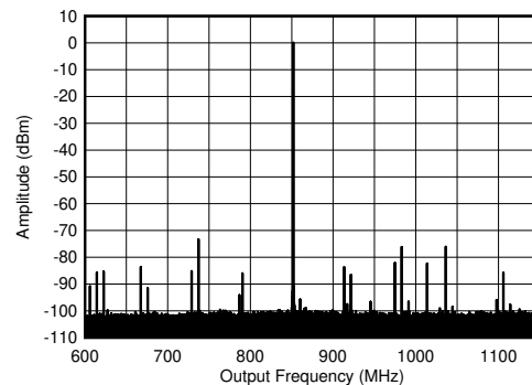
Figure 5-352. TX Single Tone (-12 dBFS) Output Spectrum at 0.85 GHz ( \pm 300 MHz)
