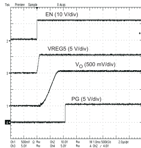
Figure 8-7. Startup Waveform
