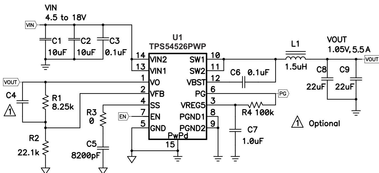
Figure 8-1. Schematic Diagram for This Design Example
