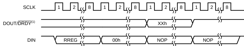
Figure 76. DOUT/DRDY Forced High after Reading Register Data
