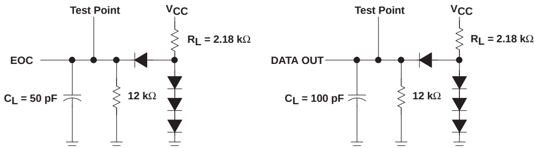
Figure 7. Load Circuits
