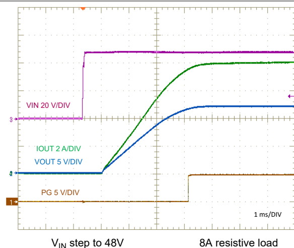
Figure 7-24. Start-Up Characteristic
