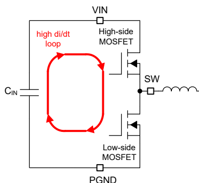
Figure 7-28. Input Current Loop
