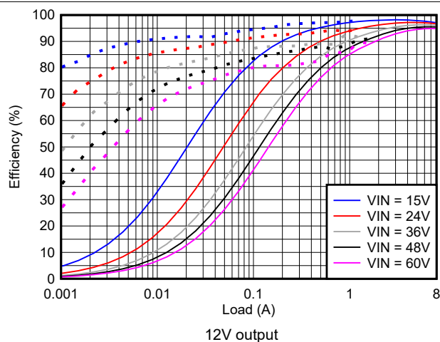
Figure 7-21. Efficiency versus I_{OUT} , Log Scale
