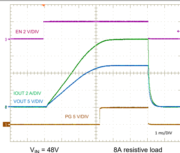
Figure 7-25. EN Start-Up Characteristic
