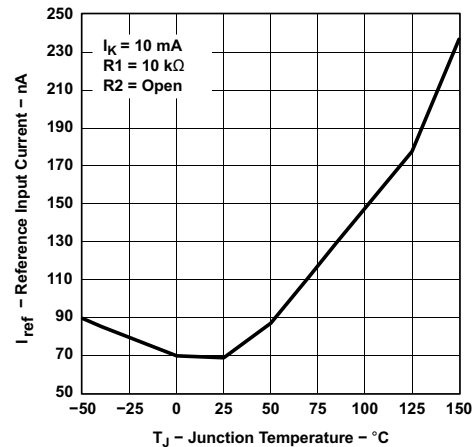
Figure 5-2. Reference Input Current vs Junction Temperature
