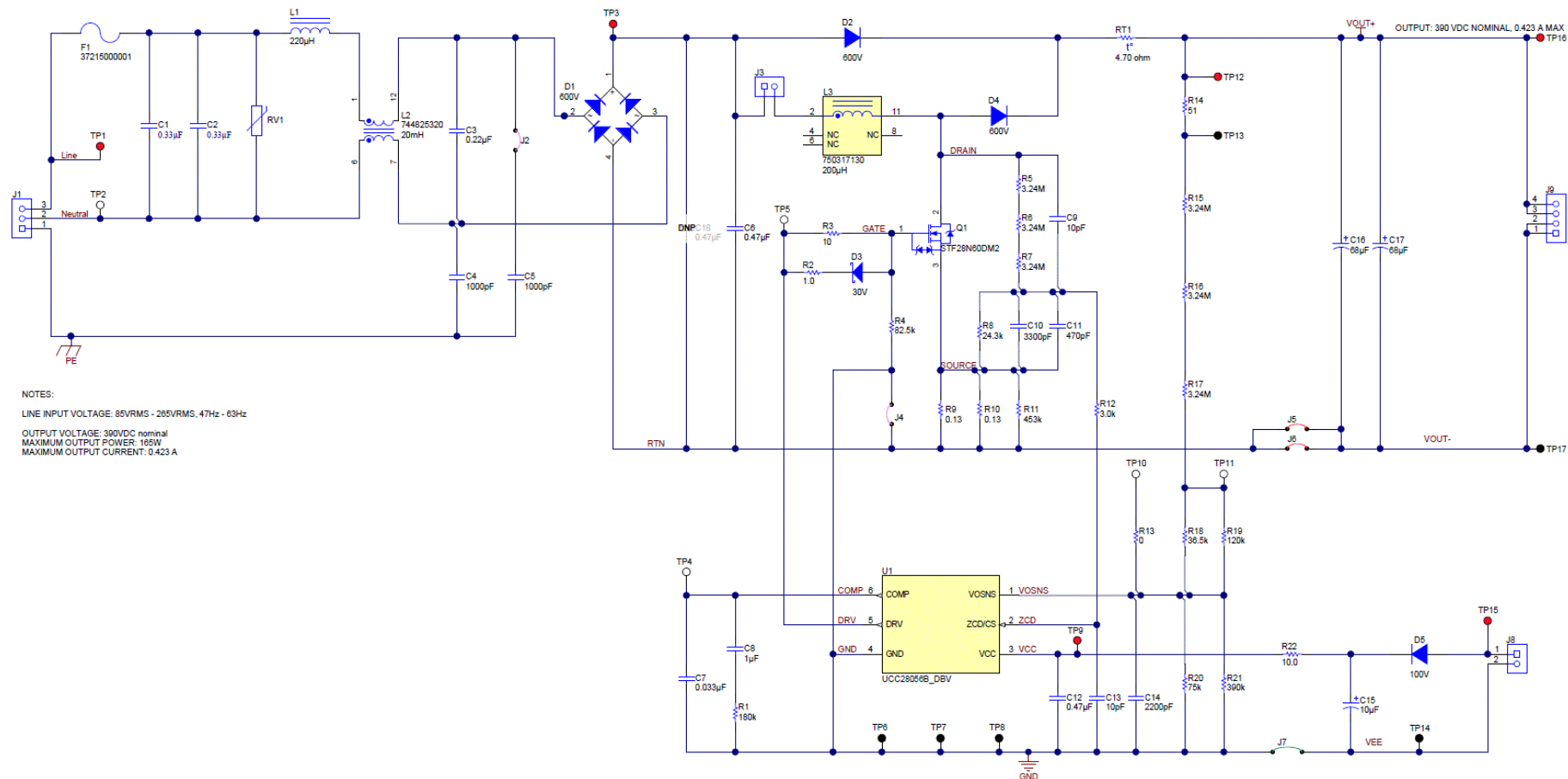
Figure 26. Typical Application Circuit for 165-W Pre-Regulator
