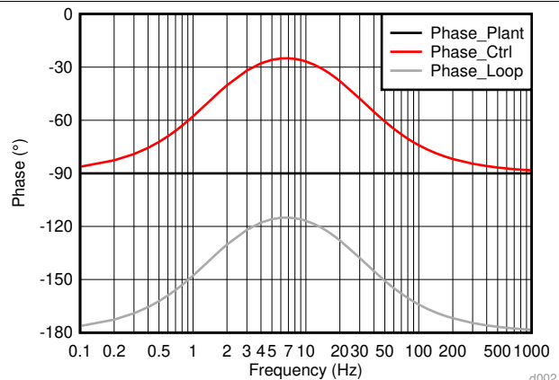
Figure 32. Phase vs Frequency
