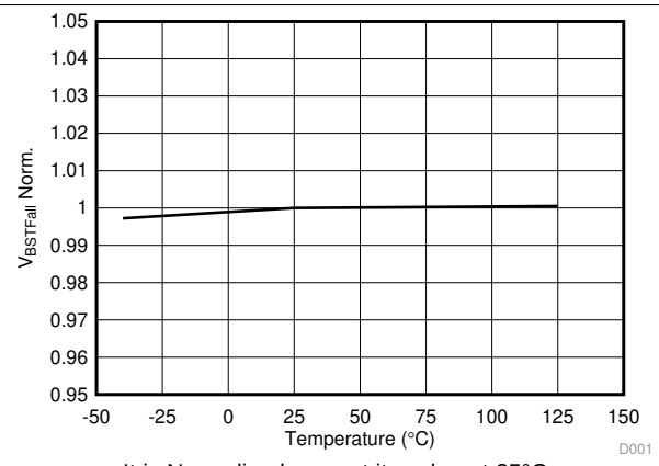
Figure 12. Burst Mode Falling Threshold vs Temperature
