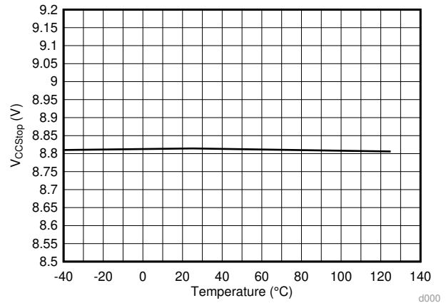
Figure 2. VCCStop Threshold vs Temperature
