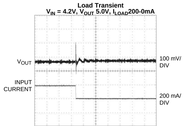
10 \mu s /DIV Figure 23.
