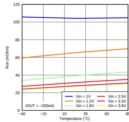
Figure 4. Temperature vs. R_{ON}
