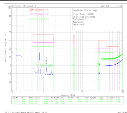
Figure 9-46. Conducted EMI versus CISPR25 Class 5 Limits (Green: Peak Signal, Blue: Average Signal)
