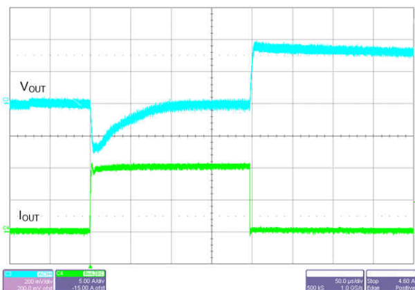
V_{OUT} = 5\text{ V} F_{SW} = 400\text{ kHz} Auto mode I_{OUT} = 10\text{ mA to } 10\text{ A to } 10\text{ mA} V_{IN} = 13.5\text{ V} T_R = T_F = 1\text{ }\mu\text{s}
