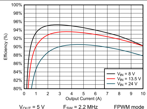
Figure 9-10. Efficiency
