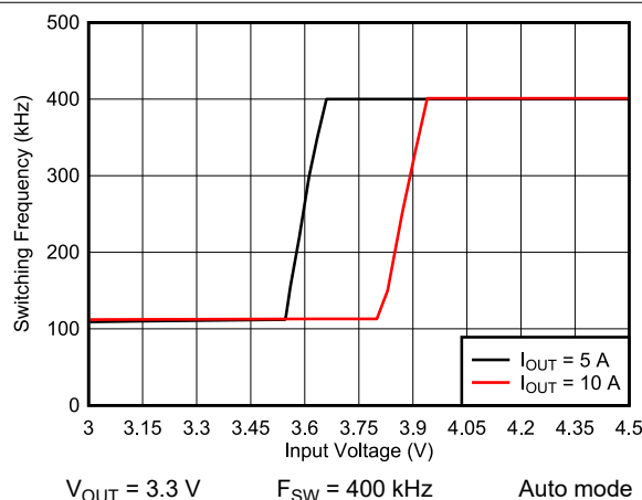
Figure 9-26. Frequency Dropout
