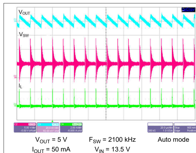
Figure 9-29. Switching Waveform and V_{OUT} Ripple
