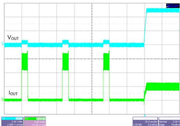
V_{OUT} = 5\text{ V} F_{SW} = 2100\text{ kHz} FPWM mode I_{OUT} = \text{Short Circuit to } 5\text{ A} V_{IN} = 13.5\text{ V}
