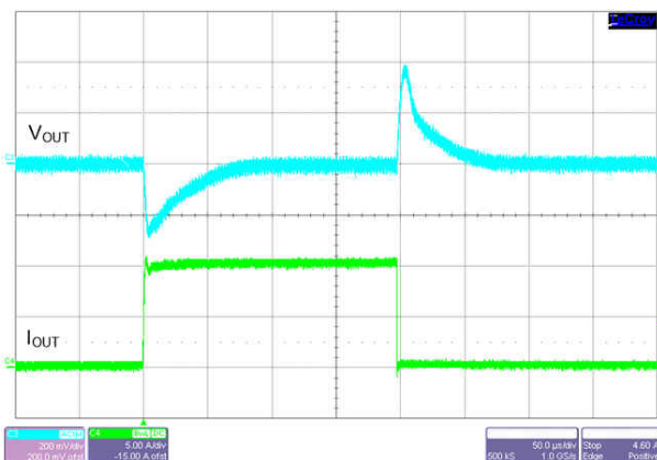
V_{OUT} = 5\text{ V} F_{SW} = 400\text{ kHz} FPWM mode I_{OUT} = 10\text{ mA to } 10\text{ A to } 10\text{ mA} V_{IN} = 13.5\text{ V} T_R = T_F = 1\text{ }\mu\text{s}
