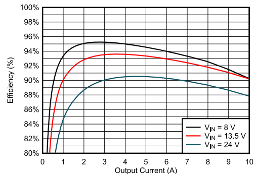
EVM Efficiency: V_{OUT} = 5\text{ V} , F_{SW} = 2.2\text{ MHz}
