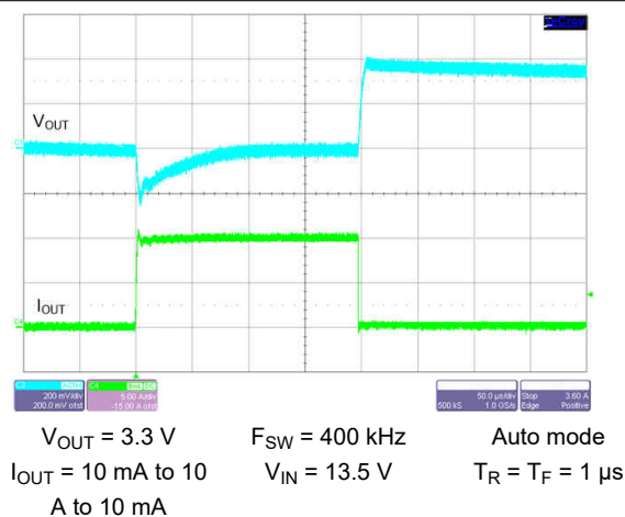
Figure 9-41. Load Transient
