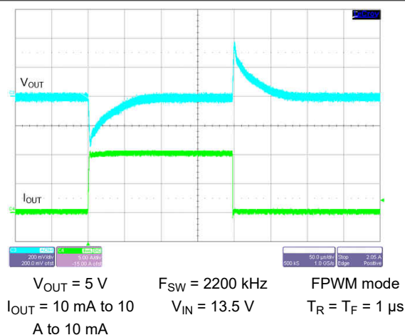
Figure 9-43. Load Transient
