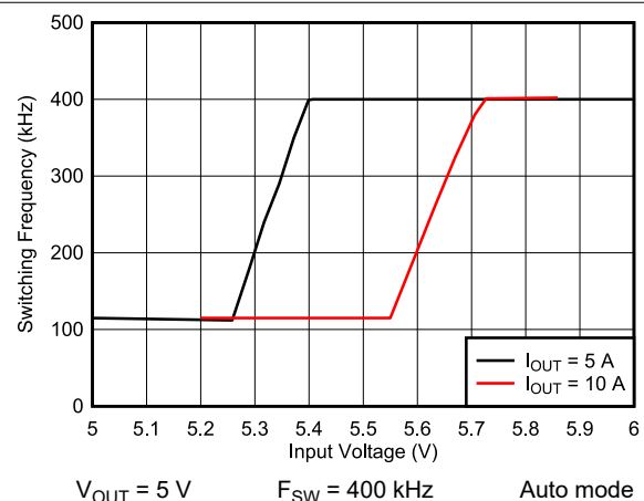
Figure 9-25. Frequency Dropout
