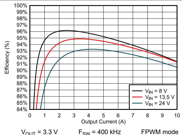
Figure 9-8. Efficiency
