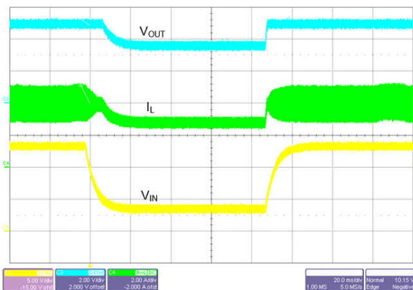
V_{OUT} = 5\text{ V} F_{SW} = 2100\text{ kHz} FPWM mode I_{OUT} = 4\text{ A} V_{IN} = 13.5\text{ V to } 4\text{ V to } 13.5\text{ V}
