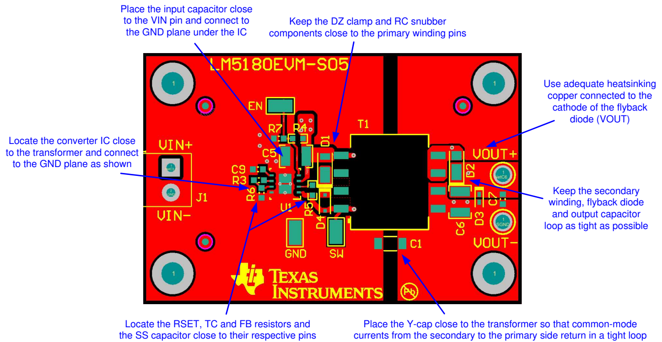
Figure 54. Single-Output PCB Layout
