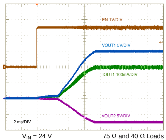
Figure 40. ENABLE ON Characteristic
