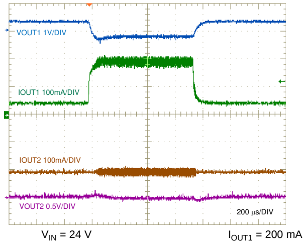
Figure 43. Output 1 Load Transient, 50 mA to 200 mA
