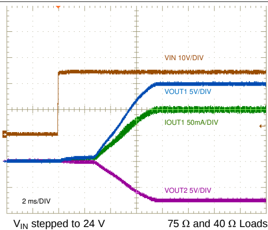
Figure 39. Start-Up Characteristic
