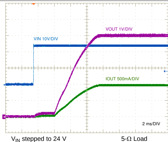
Figure 28. Start-up Characteristic
