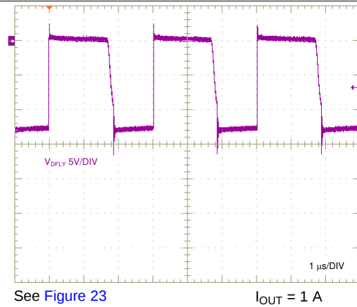
Figure 4. Flyback Diode Switching Waveform in BCM
