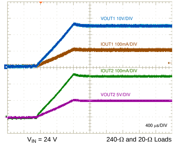
Figure 49. Recovery From Short Circuit
