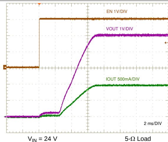
Figure 29. Enable ON Characteristic
