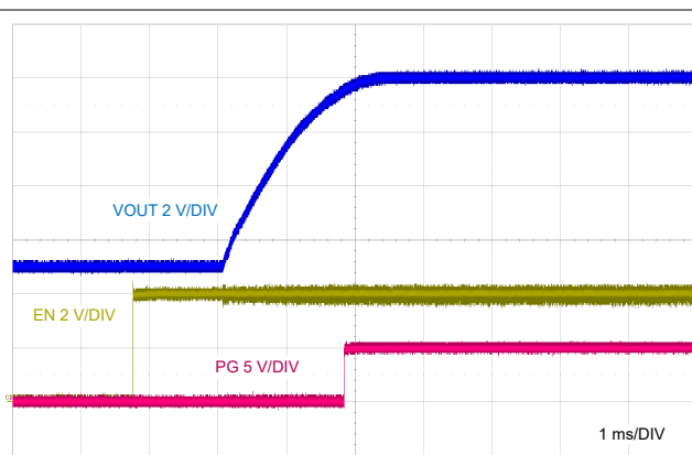
Figure 9-26. EN Start-Up Pre-bias Characteristic
