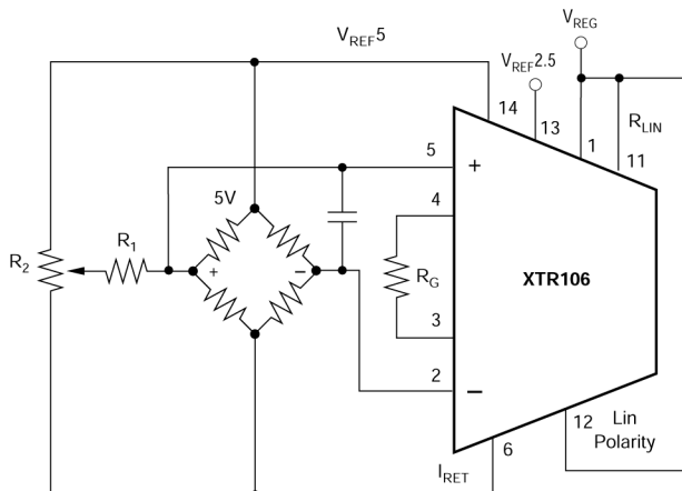
Figure 6-4. Connection if No Linearity Correction is Desired, V_{REF} = 5V
