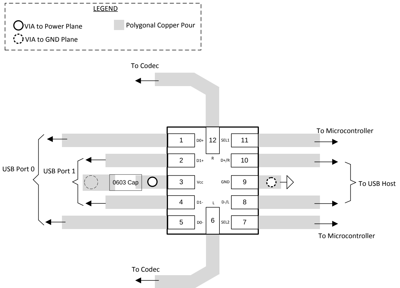
Figure 21. Layout Schematic
