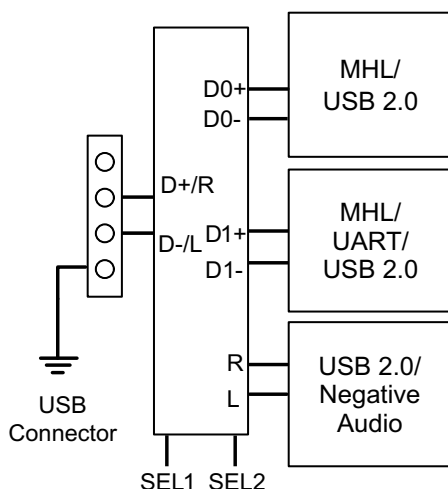
Simplified Block Diagram
