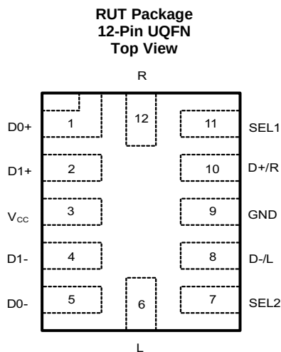
Pin Functions
