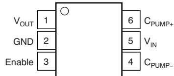
DDC PACKAGE (TOP VIEW)
