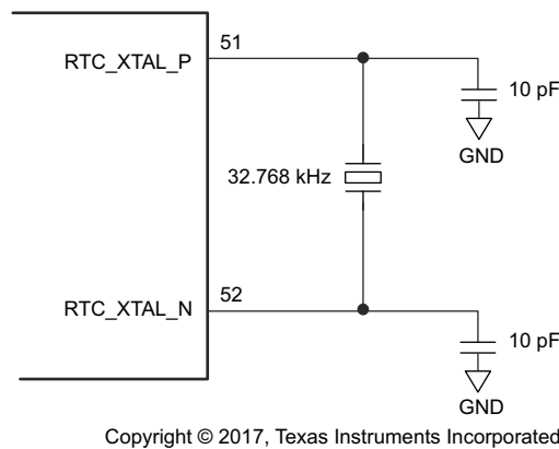
Figure 7-9. RTC Crystal Connections
