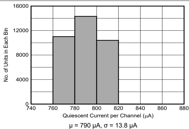
Figure 6-16. Quiescent Current Distribution
