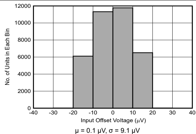
Figure 6-18. Input Offset Voltage Distribution
