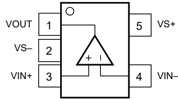
Figure 5-1. OPA863A DBV Package, 5-Pin SOT-23 (Top View)
