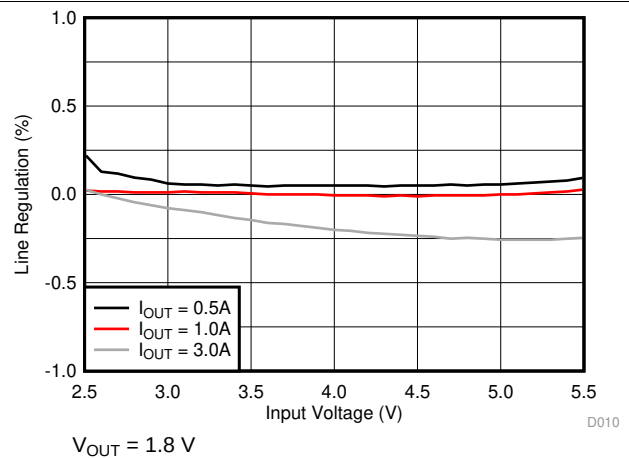
Figure 10. Line Regulation
