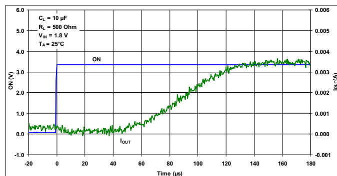
Figure 19. t_{ON} Response
