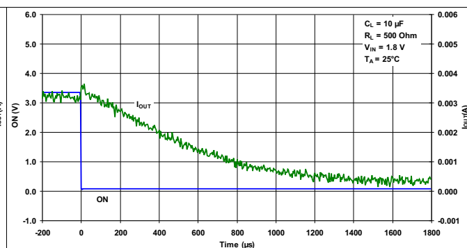
Figure 20. t_{OFF} Response
