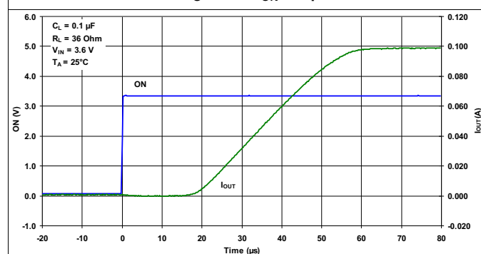
Figure 19. t_{ON} Response
