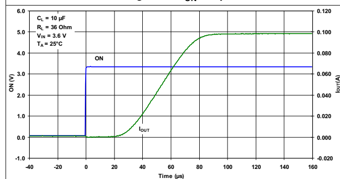
Figure 21. t_{ON} Response
