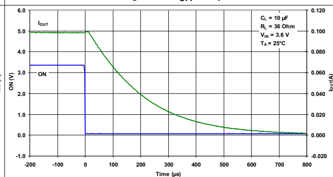
Figure 22. t_{OFF} Response
