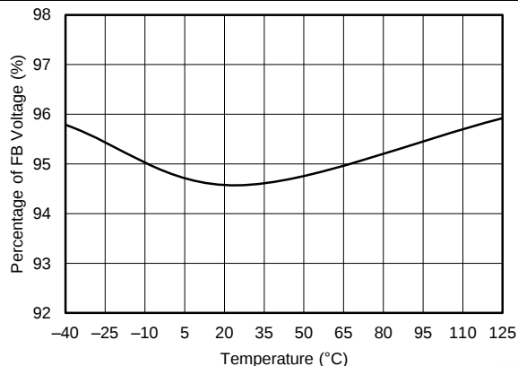
Figure 30. PGOOD UVP Rising Threshold vs Junction Temperature
