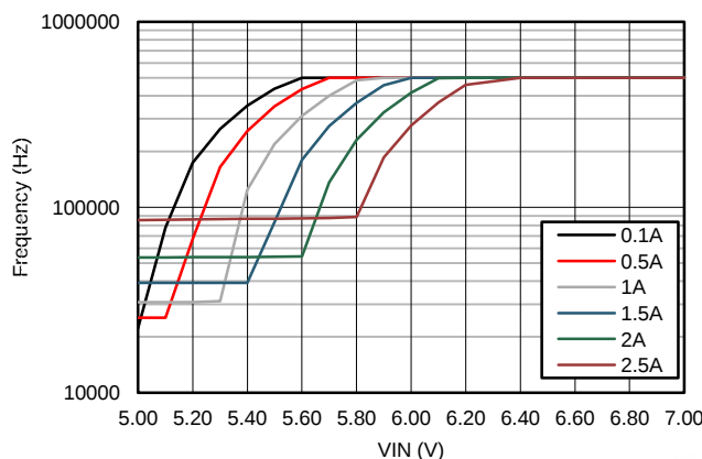
Figure 43. V_{OUT} = 5\text{ V} F_S = 500\text{ kHz} Frequency Foldback at Dropout
