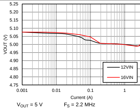
Figure 87. Output Voltage Regulation
