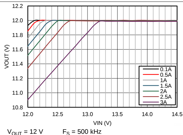
Figure 18. Dropout Curve
