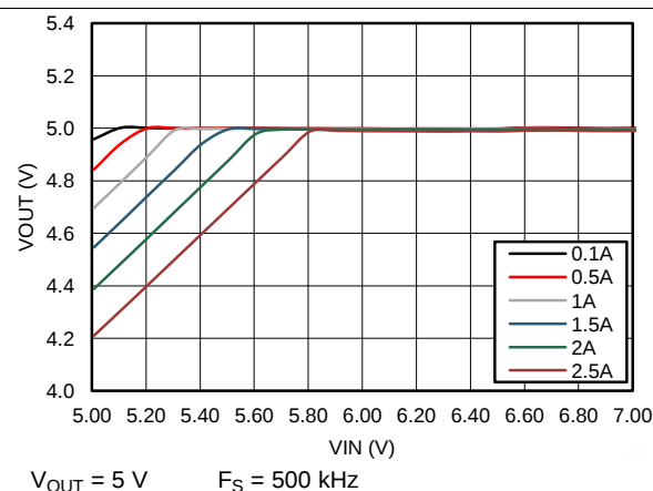
Figure 15. Dropout Curve
