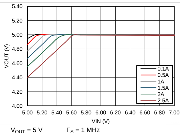
Figure 16. Dropout Curve
