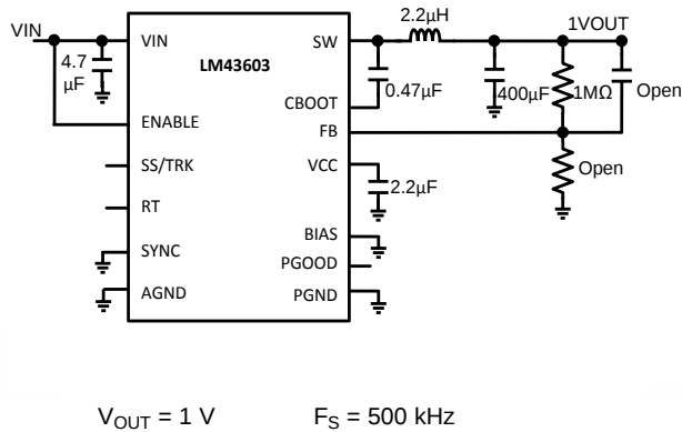
Figure 49. BOM for V_{OUT}= 1\text{V} F_S = 500\text{kHz}
