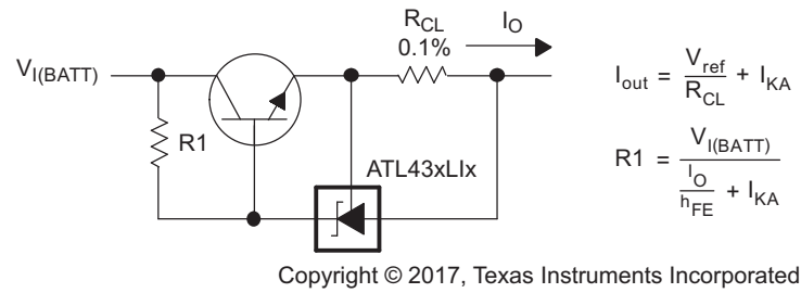
Figure 39. Precision Current Limiter
