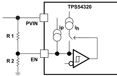
Figure 18. Adjustable PVIN UVLO, VIN ≥ 4.5 V
