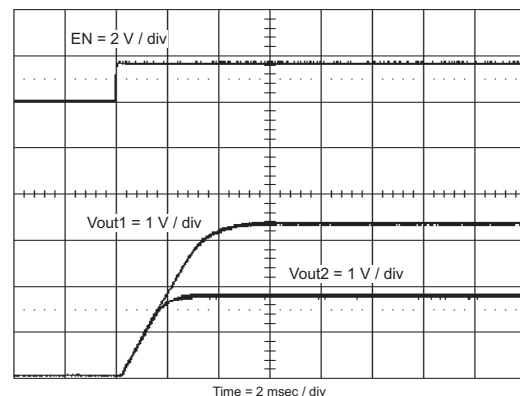
Figure 27. Simultaneous Start-Up
