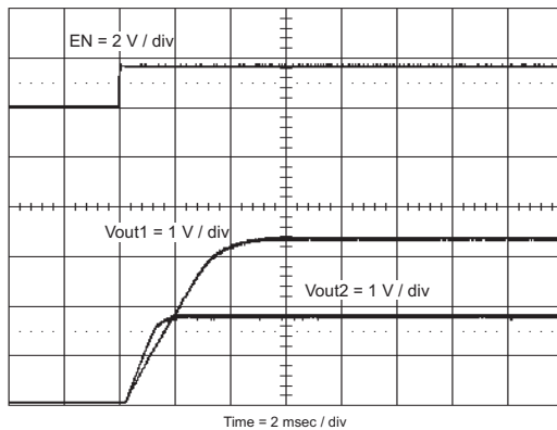
Figure 26. Ratiometric Start-Up With Vout2 Leading Vout1
