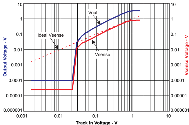
Figure 50. Tracking Performance
